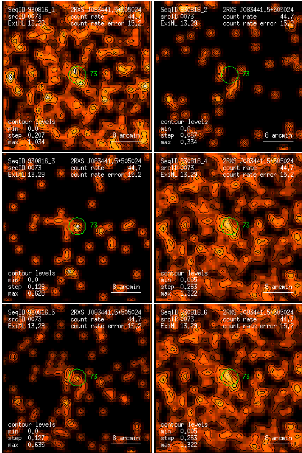
Figure 73: RASS 930816: detection 0073: band rate images, Gaussian filter: (1) PSPC channels 11 – 41, (2) 52 – 90, (3) 91 – 201, (4) 11 – 235, (5) 52 – 201, (6) 11 – 201. Broad band rates in counts/ks. Band rate contour levels in counts/ks/arcmin 2 .
