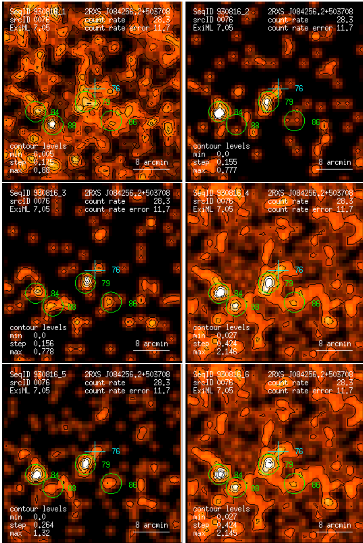
Figure 76: RASS 930816: detection 0076: band rate images, Gaussian filter: (1) PSPC channels 11 – 41, (2) 52 – 90, (3) 91 – 201, (4) 11 – 235, (5) 52 – 201, (6) 11 – 201. Broad band rates in counts/ks. Band rate contour levels in counts/ks/arcmin 2 .
