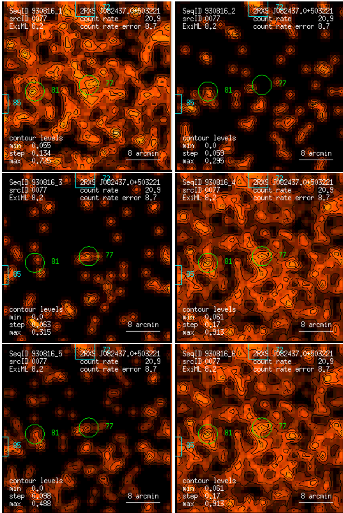
Figure 77: RASS 930816: detection 0077: band rate images, Gaussian filter: (1) PSPC channels 11 – 41, (2) 52 – 90, (3) 91 – 201, (4) 11 – 235, (5) 52 – 201, (6) 11 – 201. Broad band rates in counts/ks. Band rate contour levels in counts/ks/arcmin 2 .
