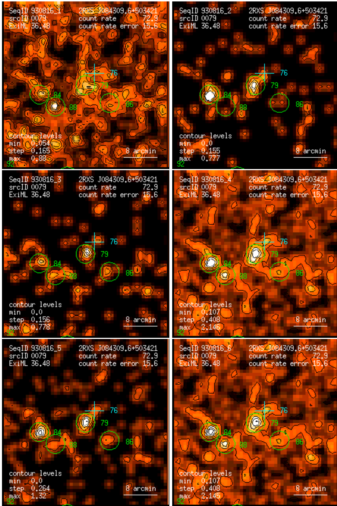
Figure 79: RASS 930816: detection 0079: band rate images, Gaussian filter: (1) PSPC channels 11 – 41, (2) 52 – 90, (3) 91 – 201, (4) 11 – 235, (5) 52 – 201, (6) 11 – 201. Broad band rates in counts/ks. Band rate contour levels in counts/ks/arcmin 2 .
