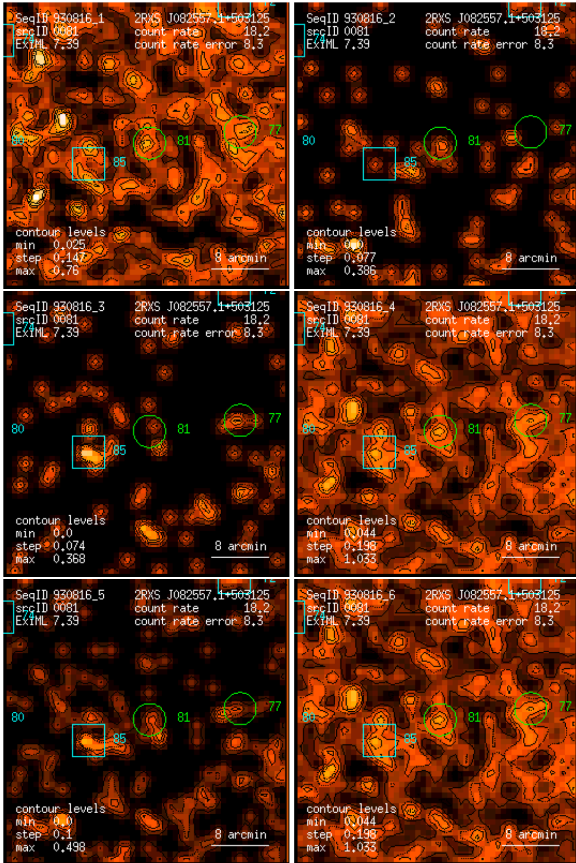
Figure 81: RASS 930816: detection 0081: band rate images, Gaussian filter: (1) PSPC channels 11 – 41, (2) 52 – 90, (3) 91 – 201, (4) 11 – 235, (5) 52 – 201, (6) 11 – 201. Broad band rates in counts/ks. Band rate contour levels in counts/ks/arcmin 2 .
