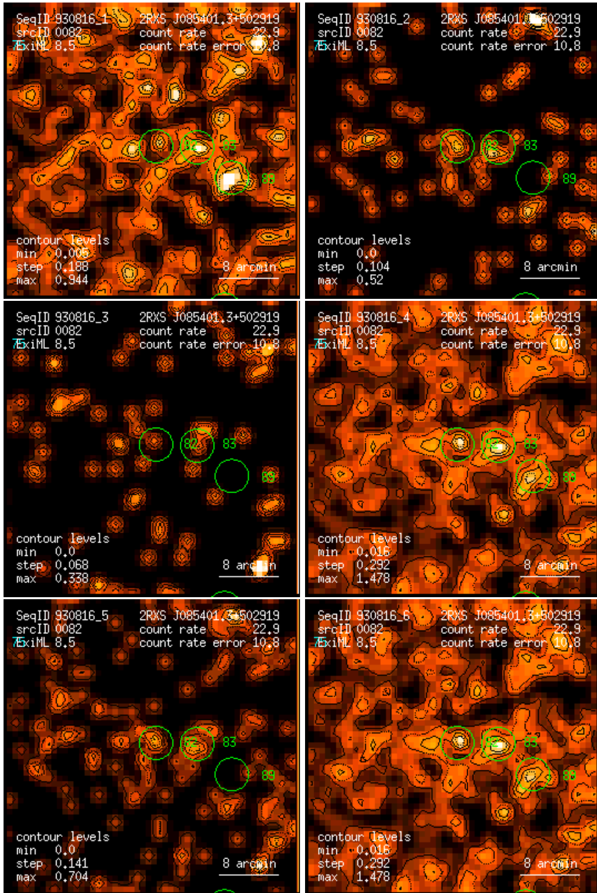
Figure 82: RASS 930816: detection 0082: band rate images, Gaussian filter: (1) PSPC channels 11 – 41, (2) 52 – 90, (3) 91 – 201, (4) 11 – 235, (5) 52 – 201, (6) 11 – 201. Broad band rates in counts/ks. Band rate contour levels in counts/ks/arcmin 2 .
