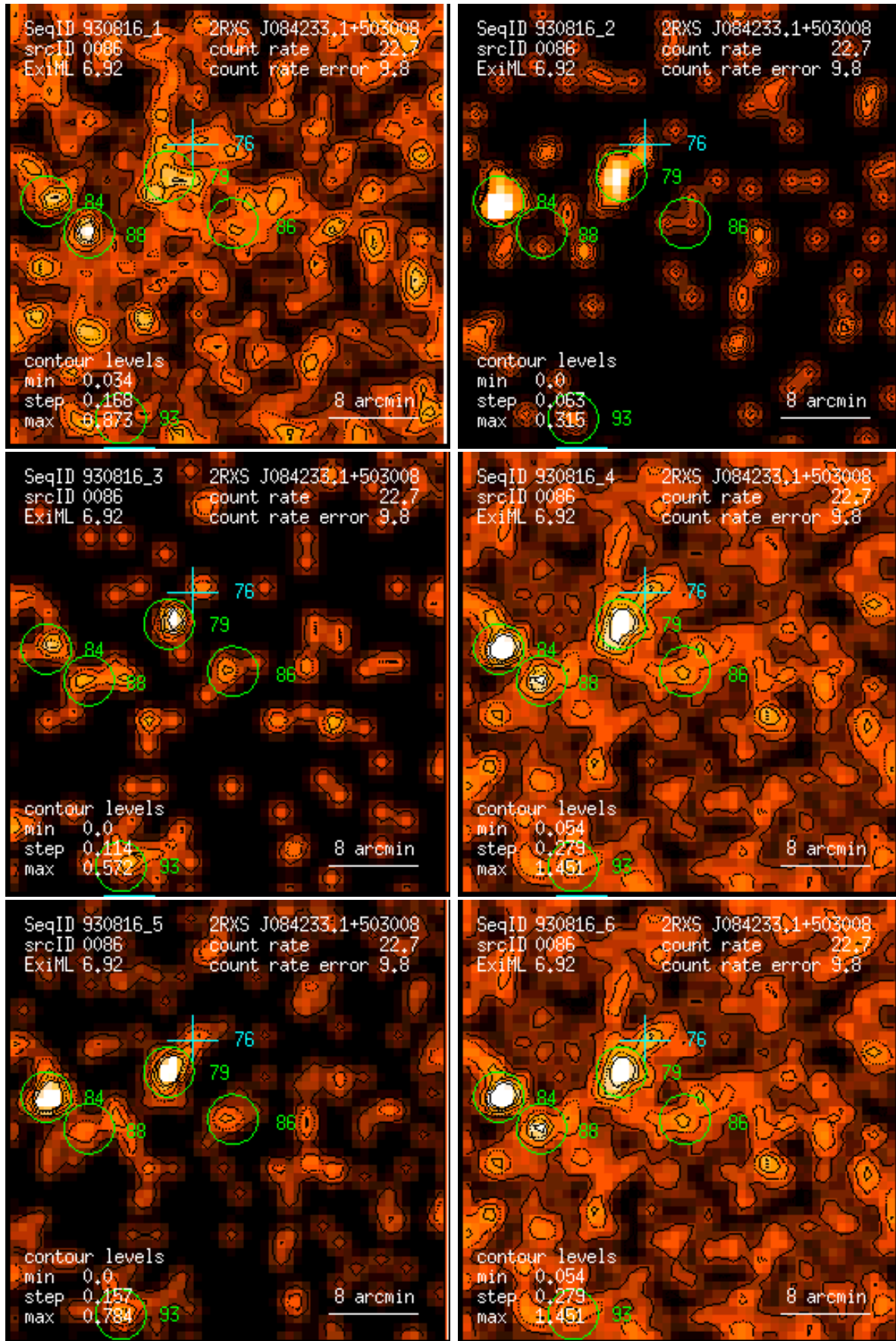
Figure 86: RASS 930816: detection 0086: band rate images, Gaussian filter: (1) PSPC channels 11 – 41, (2) 52 – 90, (3) 91 – 201, (4) 11 – 235, (5) 52 – 201, (6) 11 – 201. Broad band rates in counts/ks. Band rate contour levels in counts/ks/arcmin 2 .
