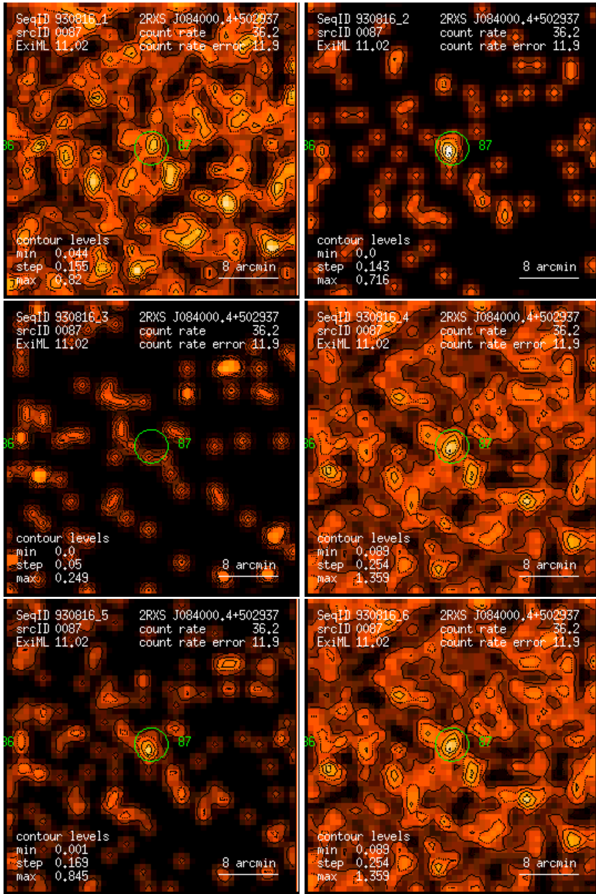
Figure 87: RASS 930816: detection 0087: band rate images, Gaussian filter: (1) PSPC channels 11 – 41, (2) 52 – 90, (3) 91 – 201, (4) 11 – 235, (5) 52 – 201, (6) 11 – 201. Broad band rates in counts/ks. Band rate contour levels in counts/ks/arcmin 2 .
