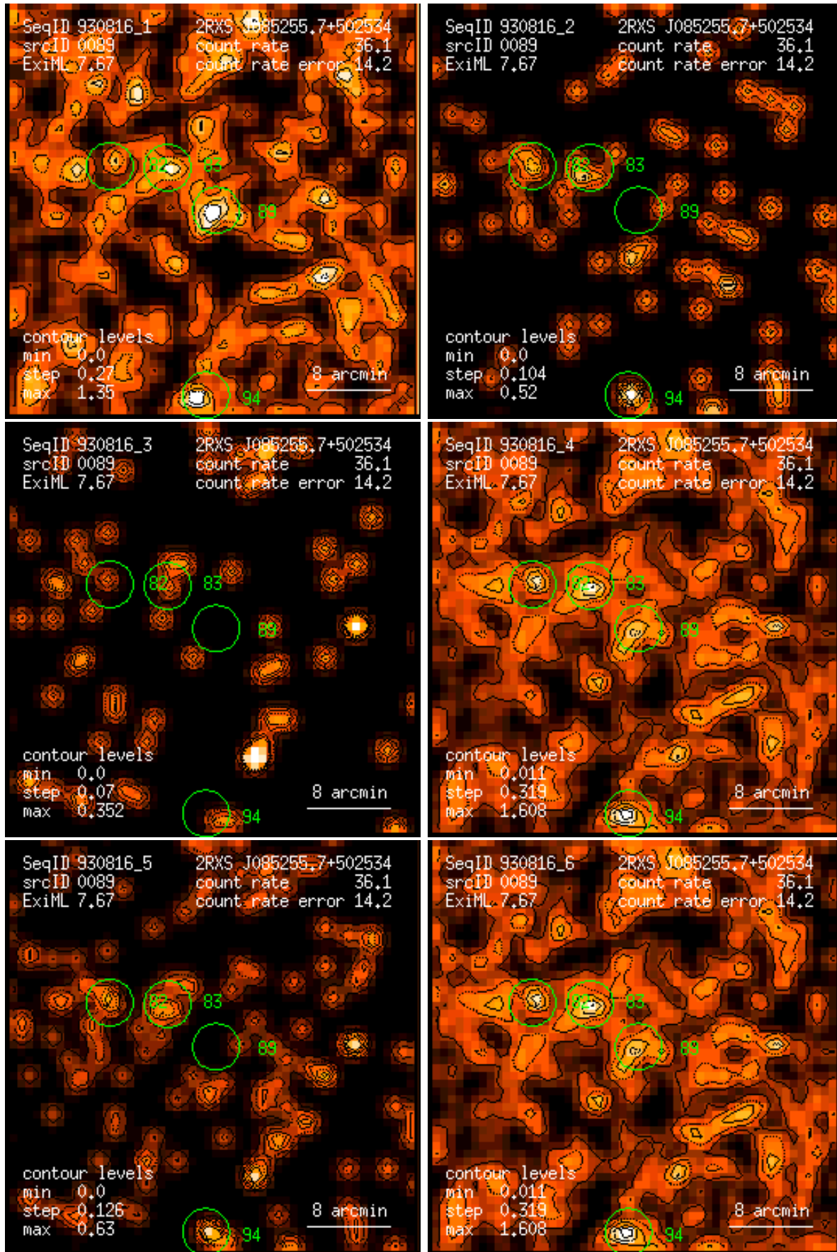
Figure 89: RASS 930816: detection 0089: band rate images, Gaussian filter: (1) PSPC channels 11 – 41, (2) 52 – 90, (3) 91 – 201, (4) 11 – 235, (5) 52 – 201, (6) 11 – 201. Broad band rates in counts/ks. Band rate contour levels in counts/ks/arcmin 2 .
