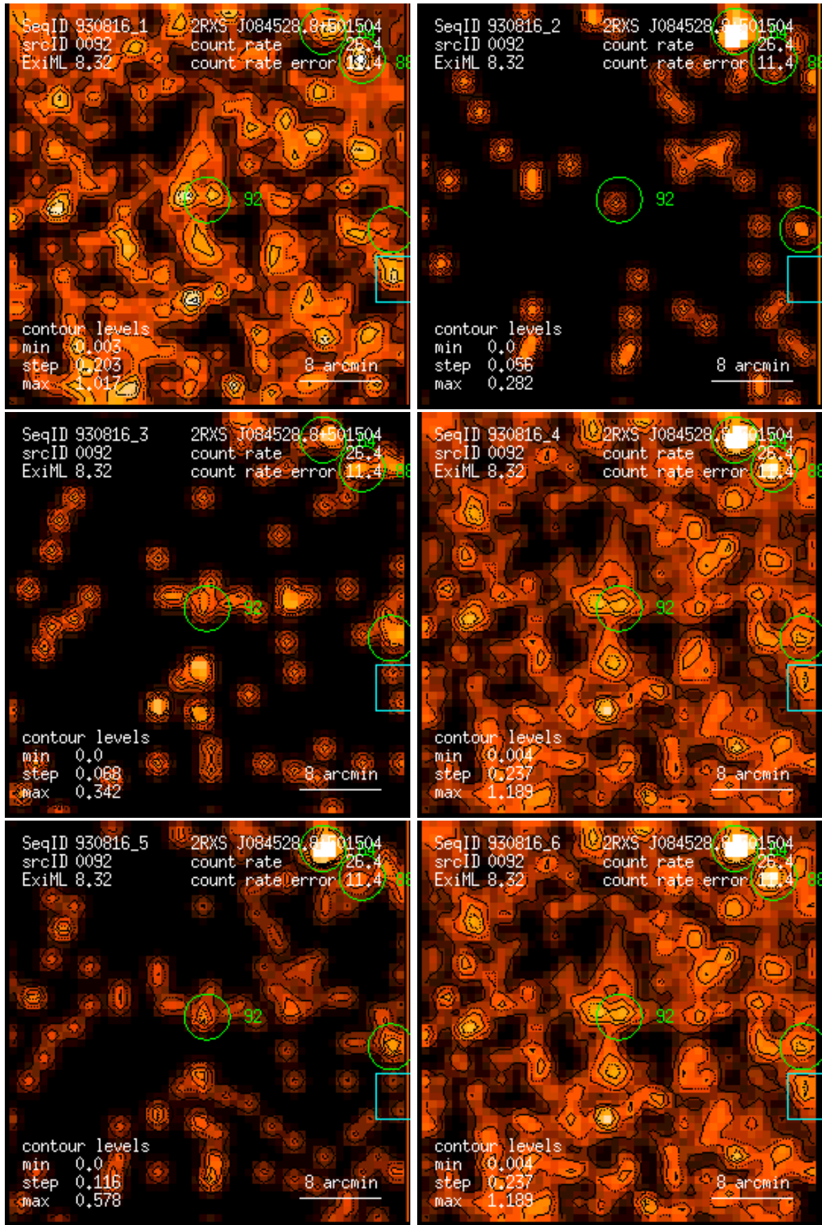
Figure 92: RASS 930816: detection 0092: band rate images, Gaussian filter: (1) PSPC channels 11 – 41, (2) 52 – 90, (3) 91 – 201, (4) 11 – 235, (5) 52 – 201, (6) 11 – 201. Broad band rates in counts/ks. Band rate contour levels in counts/ks/arcmin 2 .
