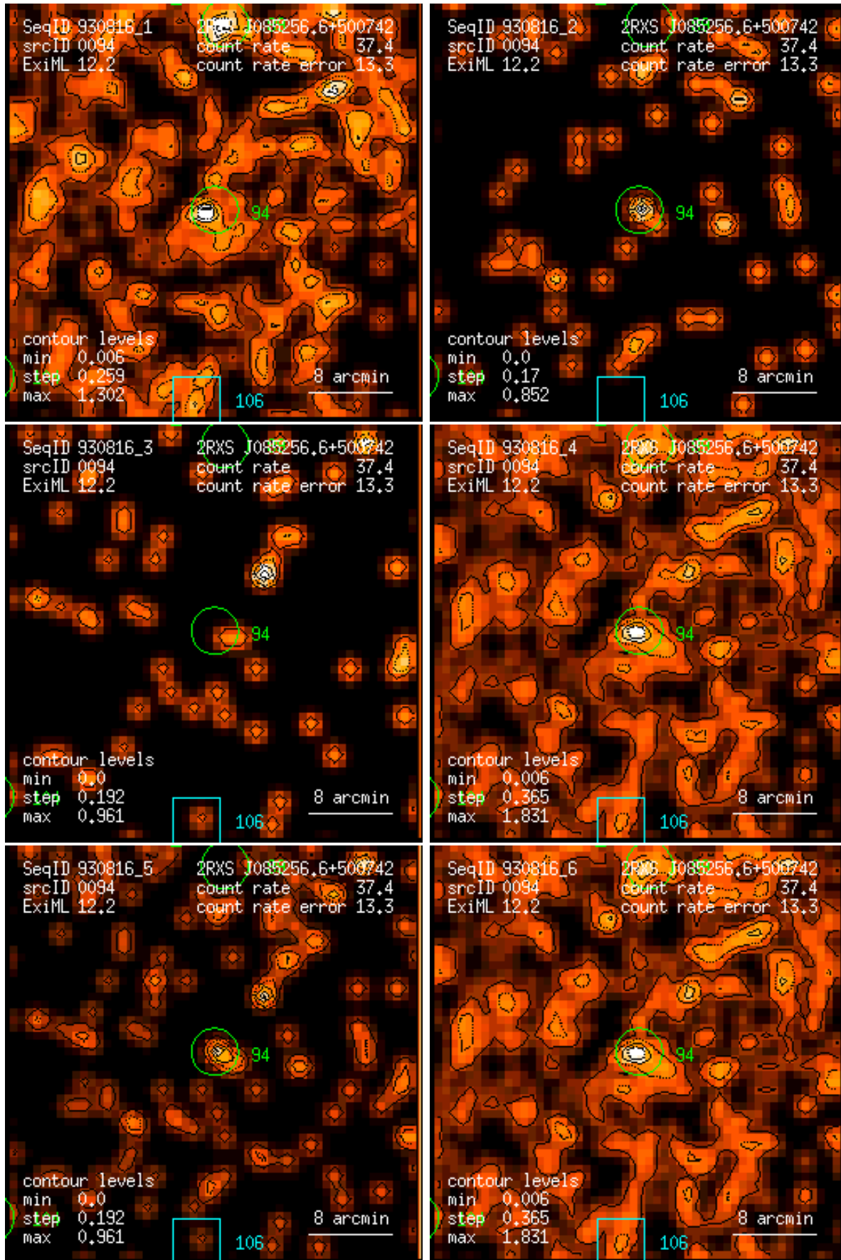
Figure 94: RASS 930816: detection 0094: band rate images, Gaussian filter: (1) PSPC channels 11 – 41, (2) 52 – 90, (3) 91 – 201, (4) 11 – 235, (5) 52 – 201, (6) 11 – 201. Broad band rates in counts/ks. Band rate contour levels in counts/ks/arcmin 2 .
