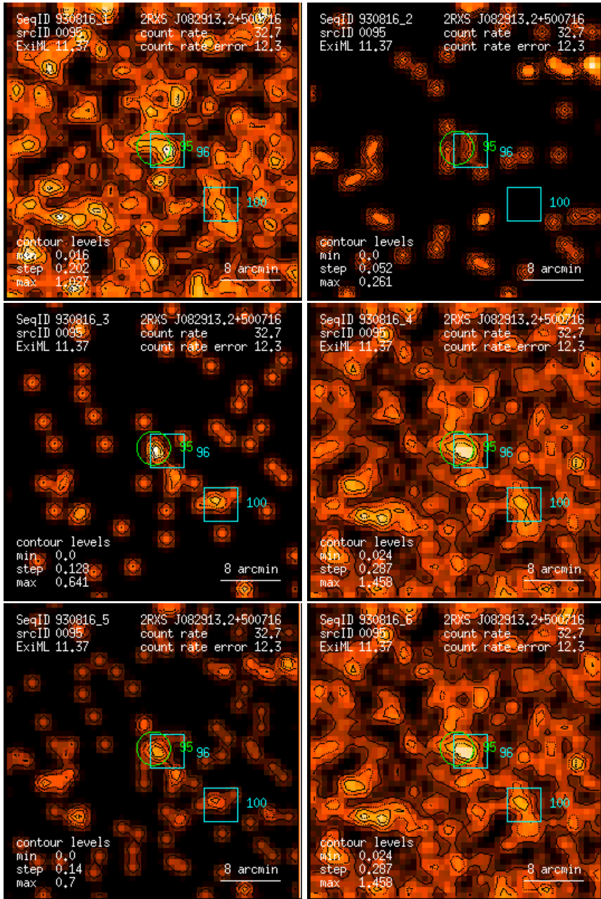
Figure 95: RASS 930816: detection 0095: band rate images, Gaussian filter: (1) PSPC channels 11 – 41, (2) 52 – 90, (3) 91 – 201, (4) 11 – 235, (5) 52 – 201, (6) 11 – 201. Broad band rates in counts/ks. Band rate contour levels in counts/ks/arcmin 2 .
