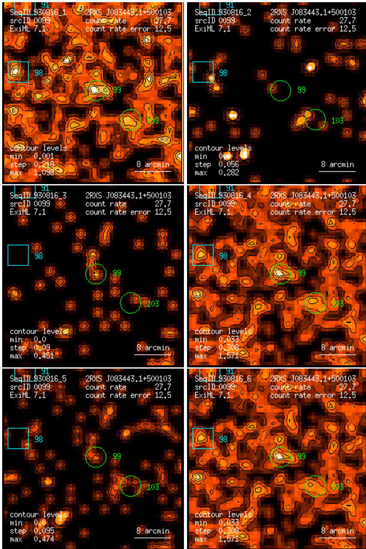
Figure 99: RASS 930816: detection 0099: band rate images, Gaussian filter: (1) PSPC channels 11 – 41, (2) 52 – 90, (3) 91 – 201, (4) 11 – 235, (5) 52 – 201, (6) 11 – 201. Broad band rates in counts/ks. Band rate contour levels in counts/ks/arcmin 2 .
