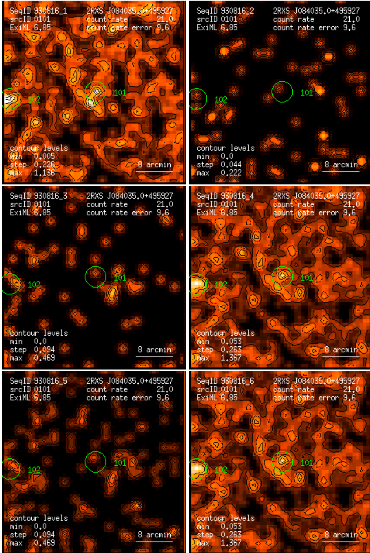
Figure 101: RASS 930816: detection 0101: band rate images, Gaussian filter: (1) PSPC channels 11 – 41, (2) 52 – 90, (3) 91 – 201, (4) 11 – 235, (5) 52 – 201, (6) 11 – 201. Broad band rates in counts/ks. Band rate contour levels in counts/ks/arcmin 2 .
