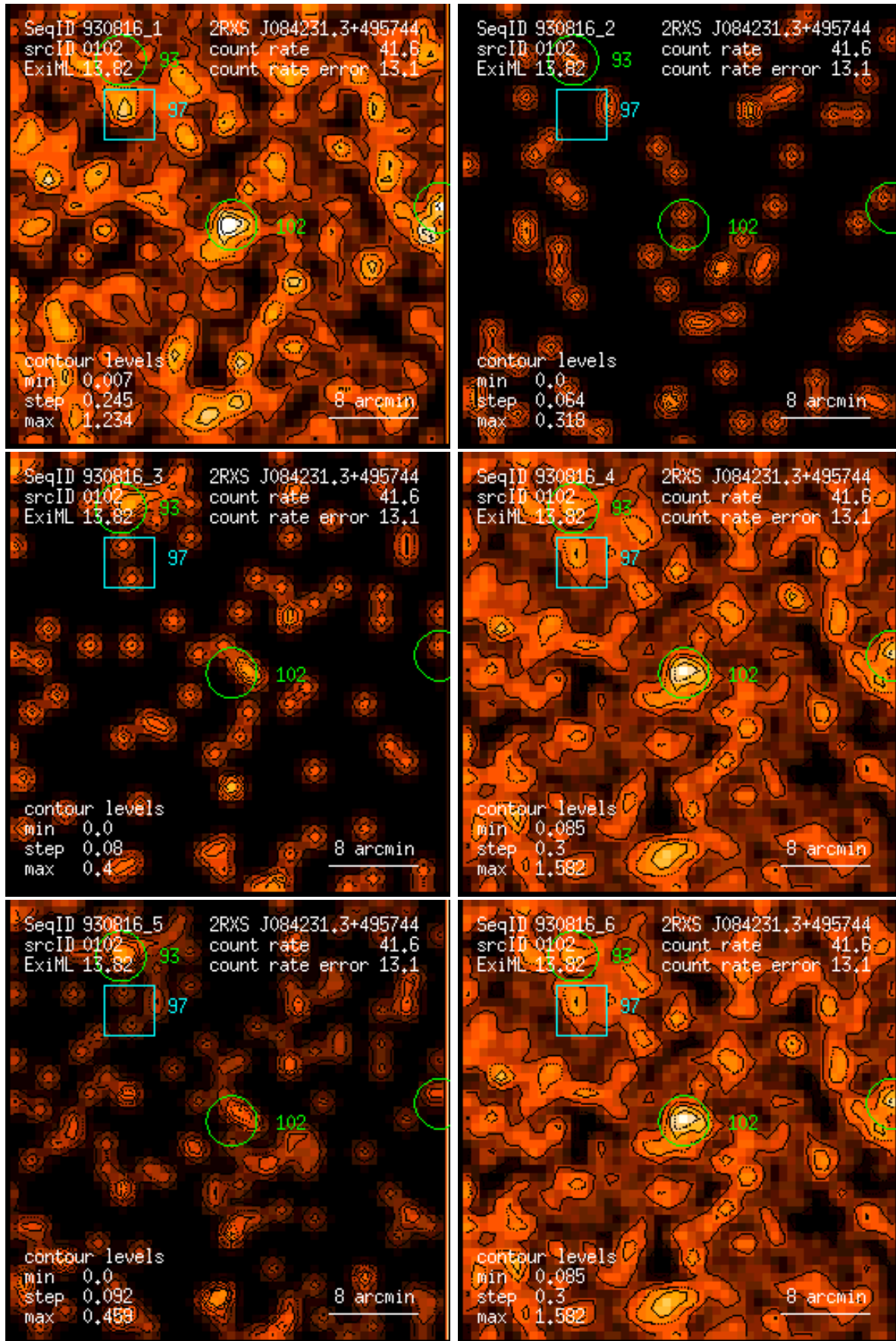
Figure 102: RASS 930816: detection 0102: band rate images, Gaussian filter: (1) PSPC channels 11 – 41, (2) 52 – 90, (3) 91 – 201, (4) 11 – 235, (5) 52 – 201, (6) 11 – 201. Broad band rates in counts/ks. Band rate contour levels in counts/ks/arcmin 2 .
