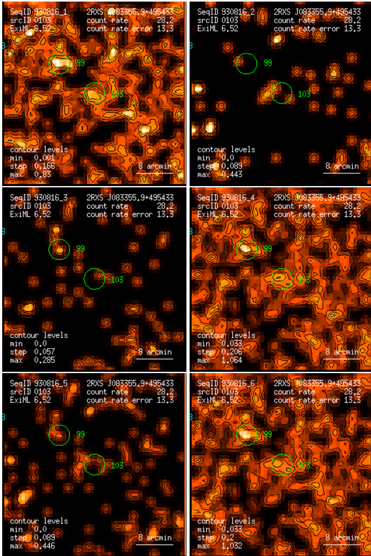
Figure 103: RASS 930816: detection 0103: band rate images, Gaussian filter: (1) PSPC channels 11 – 41, (2) 52 – 90, (3) 91 – 201, (4) 11 – 235, (5) 52 – 201, (6) 11 – 201. Broad band rates in counts/ks. Band rate contour levels in counts/ks/arcmin 2 .
