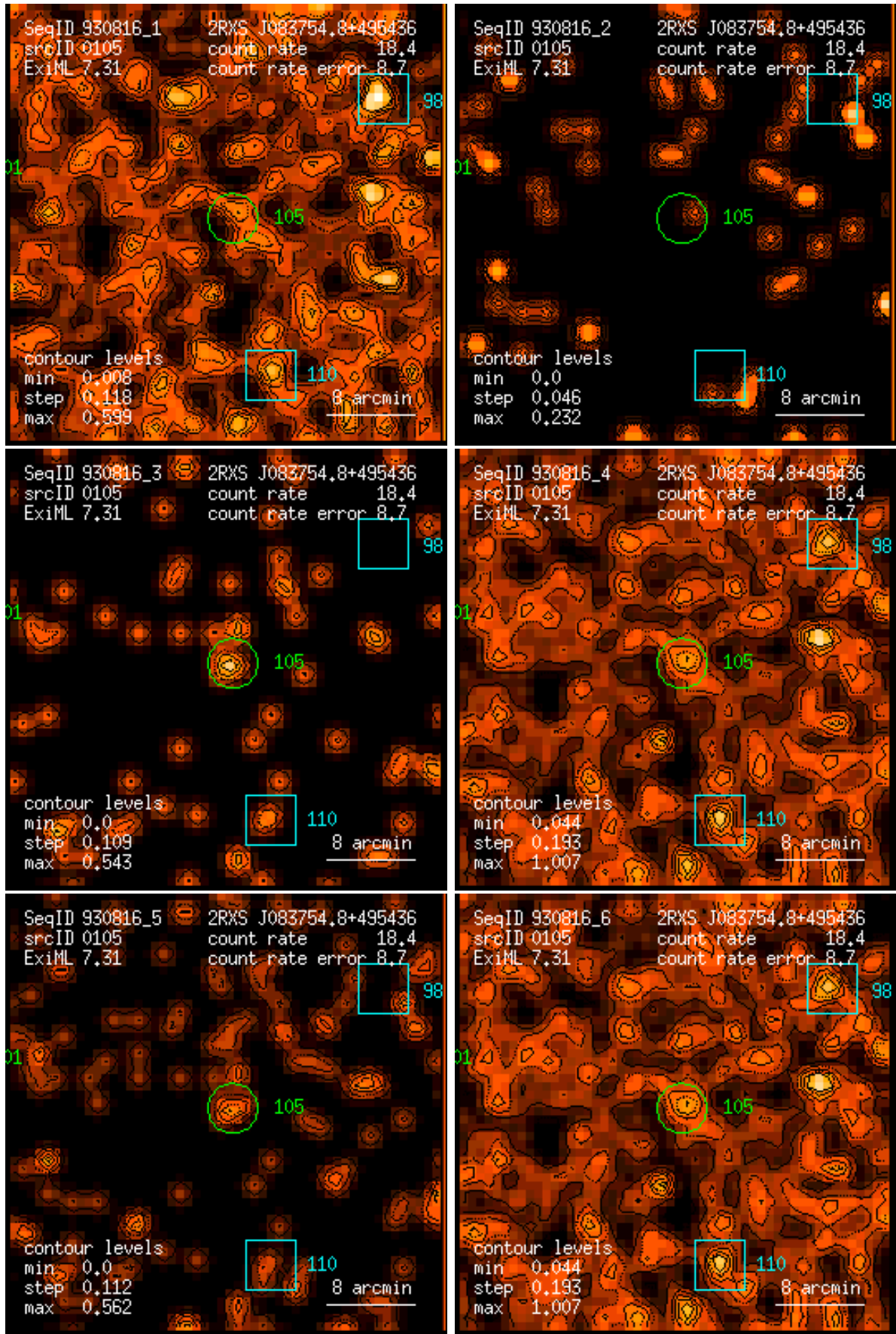
Figure 105: RASS 930816: detection 0105: band rate images, Gaussian filter: (1) PSPC channels 11 – 41, (2) 52 – 90, (3) 91 – 201, (4) 11 – 235, (5) 52 – 201, (6) 11 – 201. Broad band rates in counts/ks. Band rate contour levels in counts/ks/arcmin 2 .
