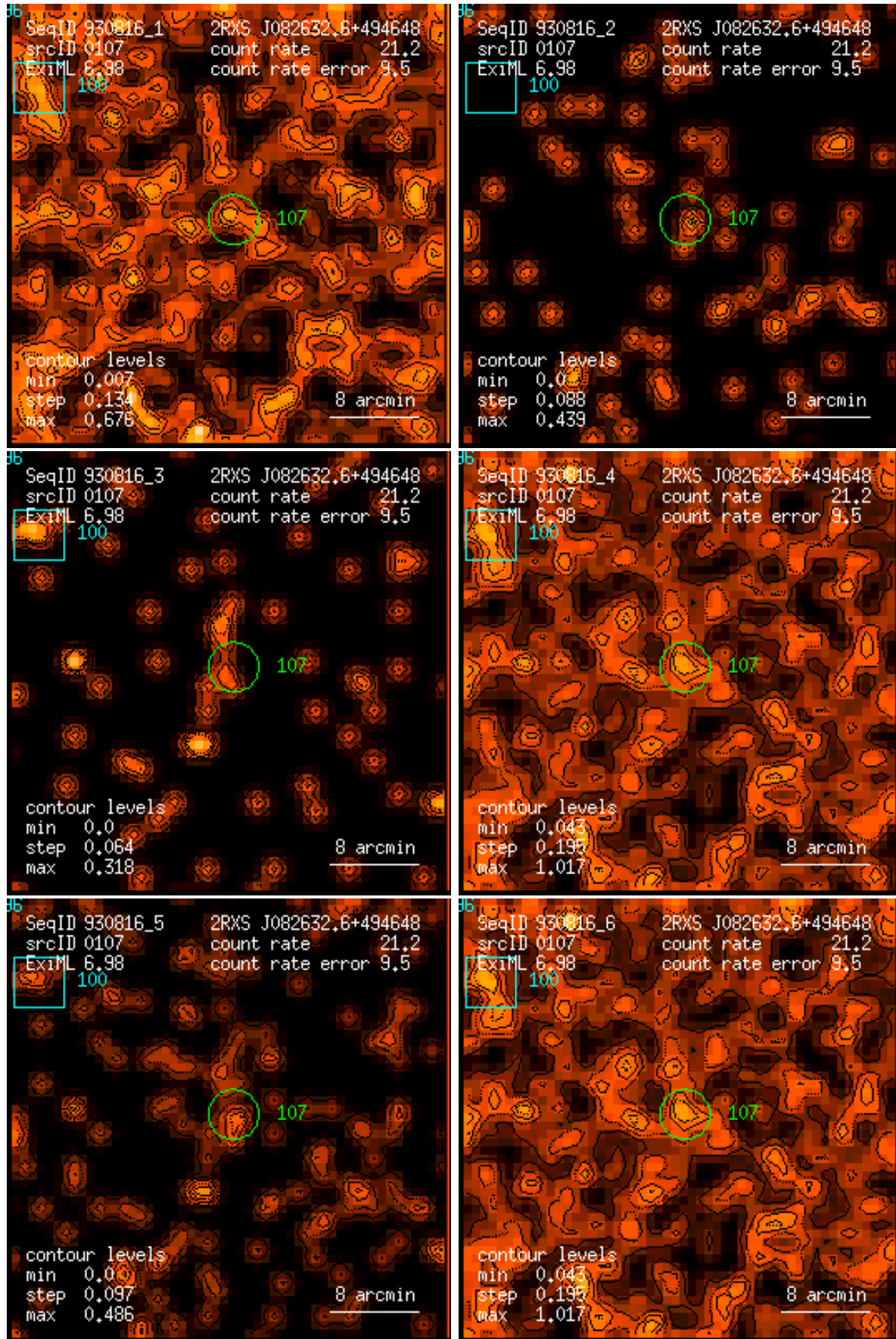
Figure 107: RASS 930816: detection 0107: band rate images, Gaussian filter: (1) PSPC channels 11 – 41, (2) 52 – 90, (3) 91 – 201, (4) 11 – 235, (5) 52 – 201, (6) 11 – 201. Broad band rates in counts/ks. Band rate contour levels in counts/ks/arcmin 2 .
