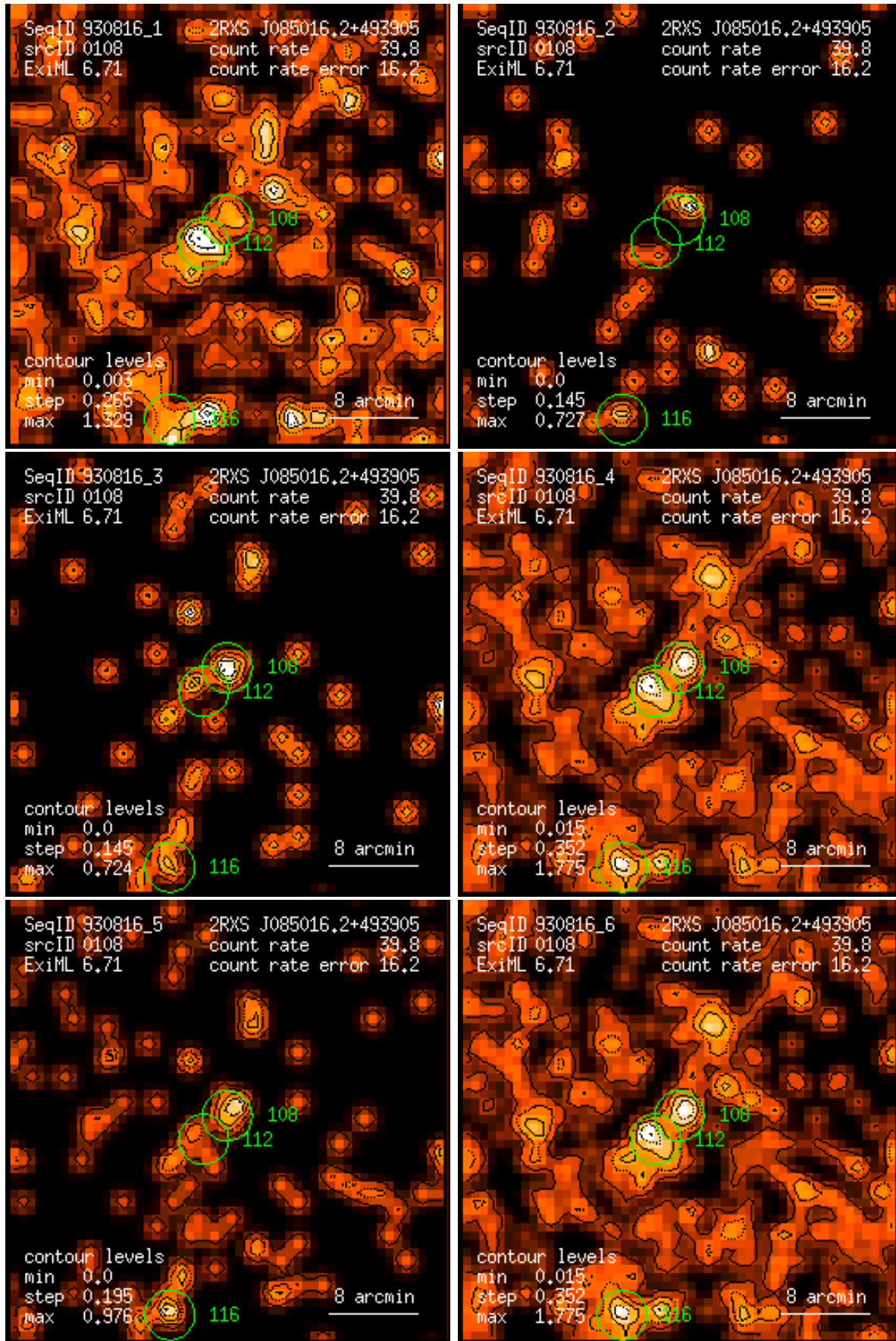
Figure 108: RASS 930816: detection 0108: band rate images, Gaussian filter: (1) PSPC channels 11 – 41, (2) 52 – 90, (3) 91 – 201, (4) 11 – 235, (5) 52 – 201, (6) 11 – 201. Broad band rates in counts/ks. Band rate contour levels in counts/ks/arcmin 2 .
