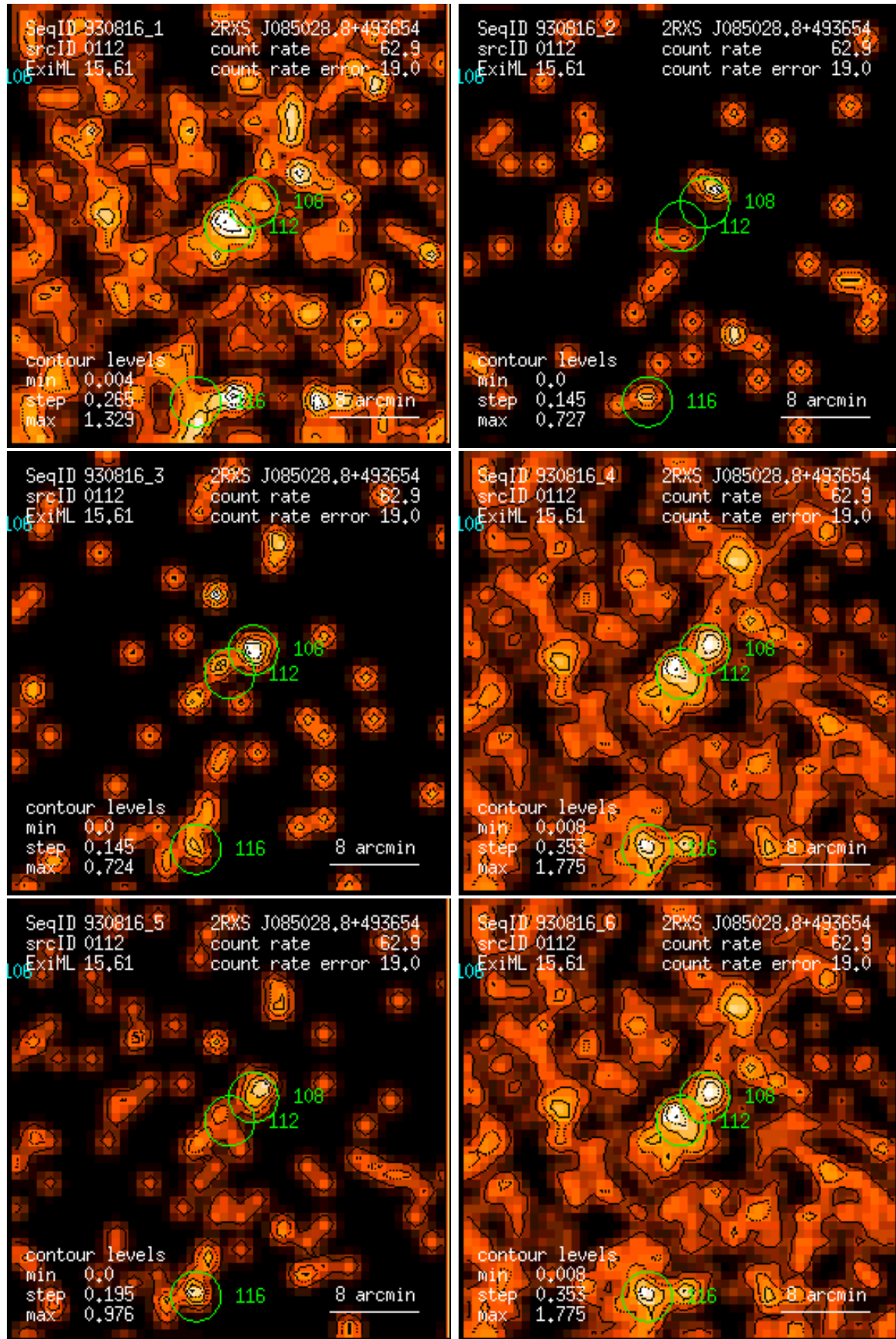
Figure 112: RASS 930816: detection 0112: band rate images, Gaussian filter: (1) PSPC channels 11 – 41, (2) 52 – 90, (3) 91 – 201, (4) 11 – 235, (5) 52 – 201, (6) 11 – 201. Broad band rates in counts/ks. Band rate contour levels in counts/ks/arcmin 2 .
