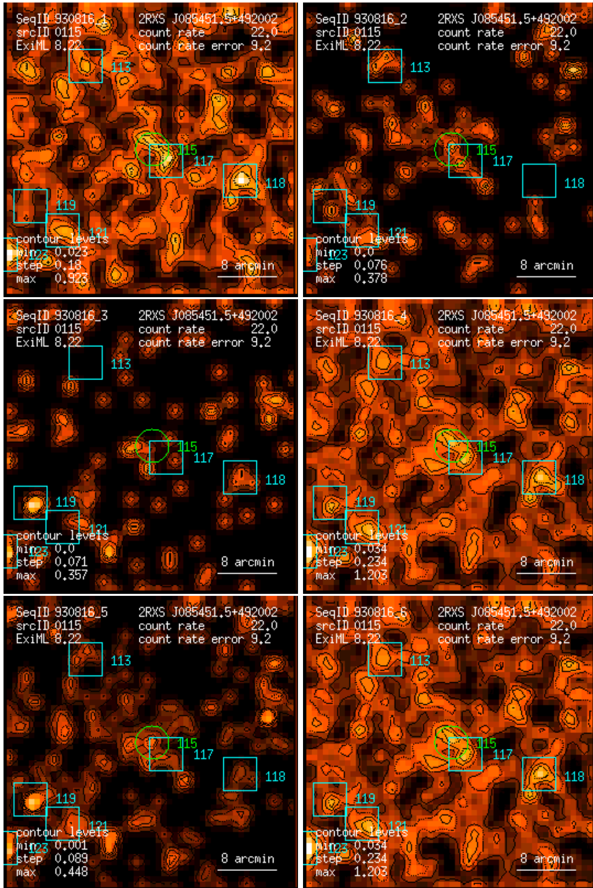
Figure 115: RASS 930816: detection 0115: band rate images, Gaussian filter: (1) PSPC channels 11 – 41, (2) 52 – 90, (3) 91 – 201, (4) 11 – 235, (5) 52 – 201, (6) 11 – 201. Broad band rates in counts/ks. Band rate contour levels in counts/ks/arcmin 2 .
