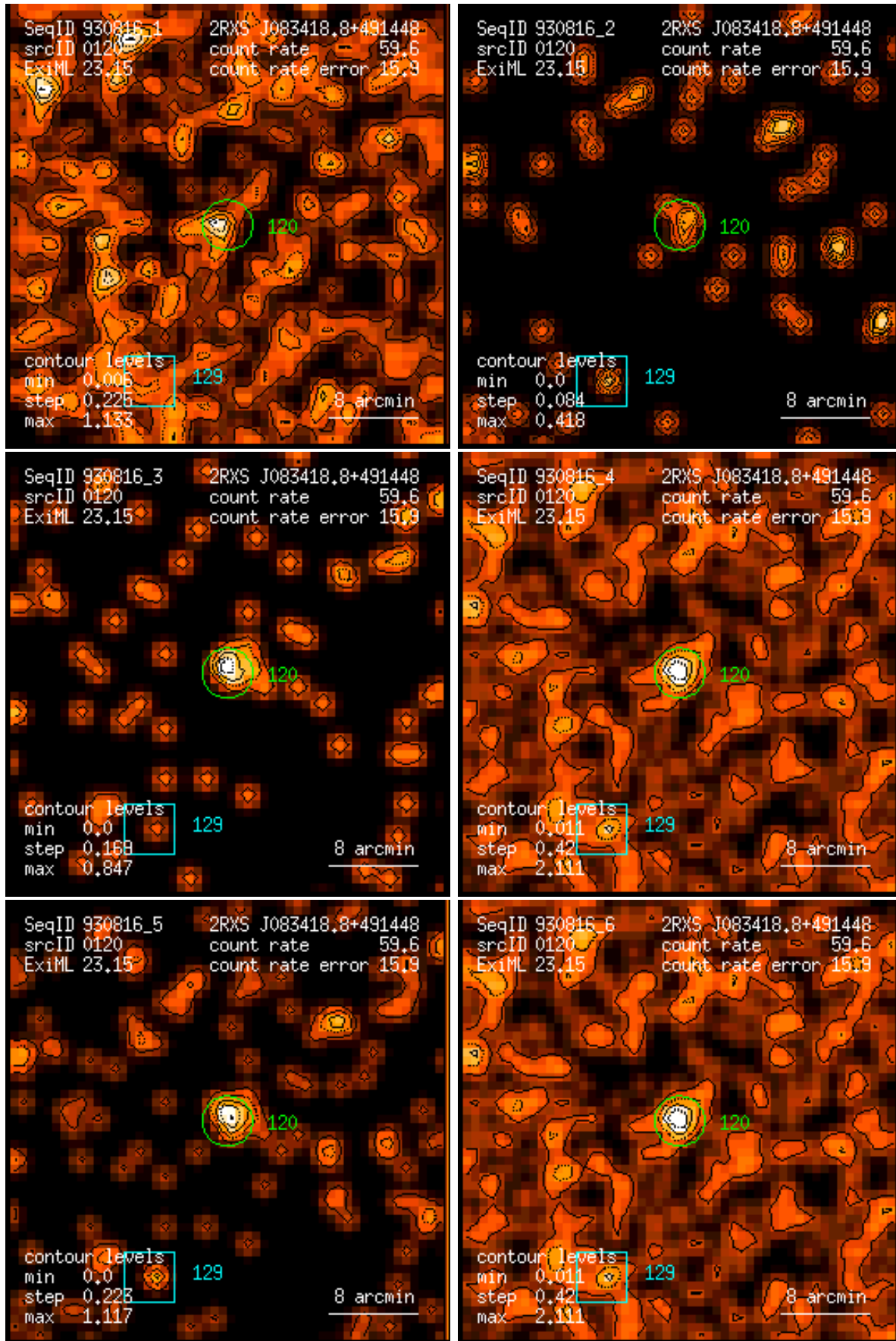
Figure 120: RASS 930816: detection 0120: band rate images, Gaussian filter: (1) PSPC channels 11 – 41, (2) 52 – 90, (3) 91 – 201, (4) 11 – 235, (5) 52 – 201, (6) 11 – 201. Broad band rates in counts/ks. Band rate contour levels in counts/ks/arcmin 2 .
