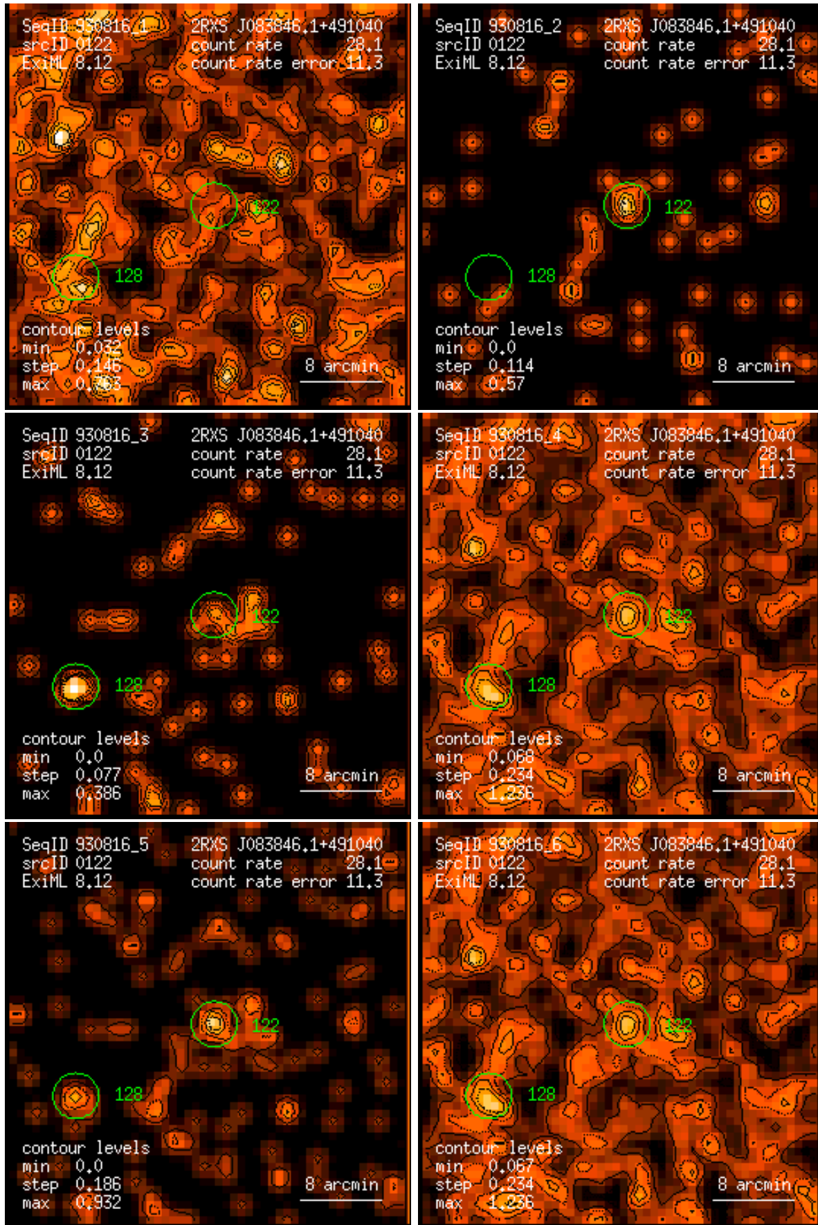
Figure 122: RASS 930816: detection 0122: band rate images, Gaussian filter: (1) PSPC channels 11 – 41, (2) 52 – 90, (3) 91 – 201, (4) 11 – 235, (5) 52 – 201, (6) 11 – 201. Broad band rates in counts/ks. Band rate contour levels in counts/ks/arcmin 2 .
