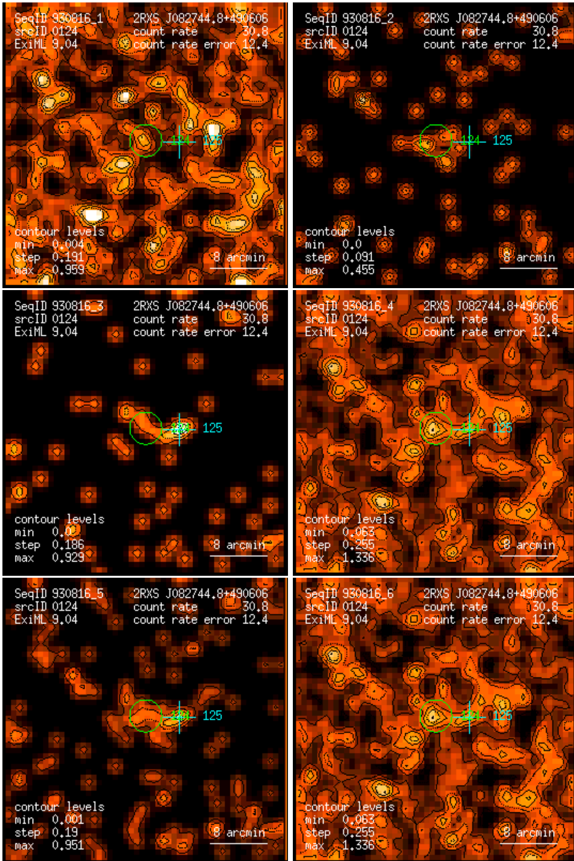
Figure 124: RASS 930816: detection 0124: band rate images, Gaussian filter: (1) PSPC channels 11 – 41, (2) 52 – 90, (3) 91 – 201, (4) 11 – 235, (5) 52 – 201, (6) 11 – 201. Broad band rates in counts/ks. Band rate contour levels in counts/ks/arcmin 2 .
