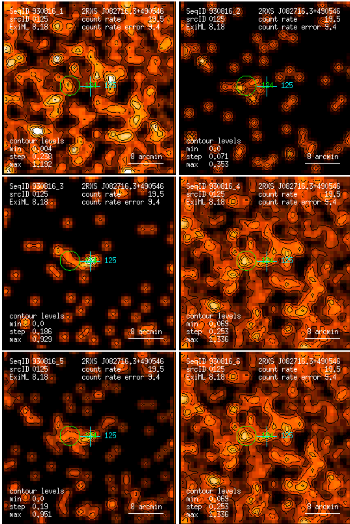
Figure 125: RASS 930816: detection 0125: band rate images, Gaussian filter: (1) PSPC channels 11 – 41, (2) 52 – 90, (3) 91 – 201, (4) 11 – 235, (5) 52 – 201, (6) 11 – 201. Broad band rates in counts/ks. Band rate contour levels in counts/ks/arcmin 2 .
