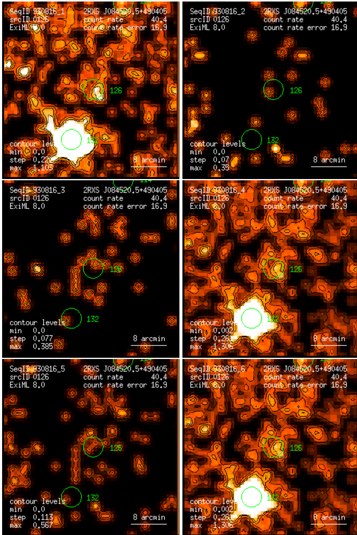
Figure 126: RASS 930816: detection 0126: band rate images, Gaussian filter: (1) PSPC channels 11 – 41, (2) 52 – 90, (3) 91 – 201, (4) 11 – 235, (5) 52 – 201, (6) 11 – 201. Broad band rates in counts/ks. Band rate contour levels in counts/ks/arcmin 2 .
