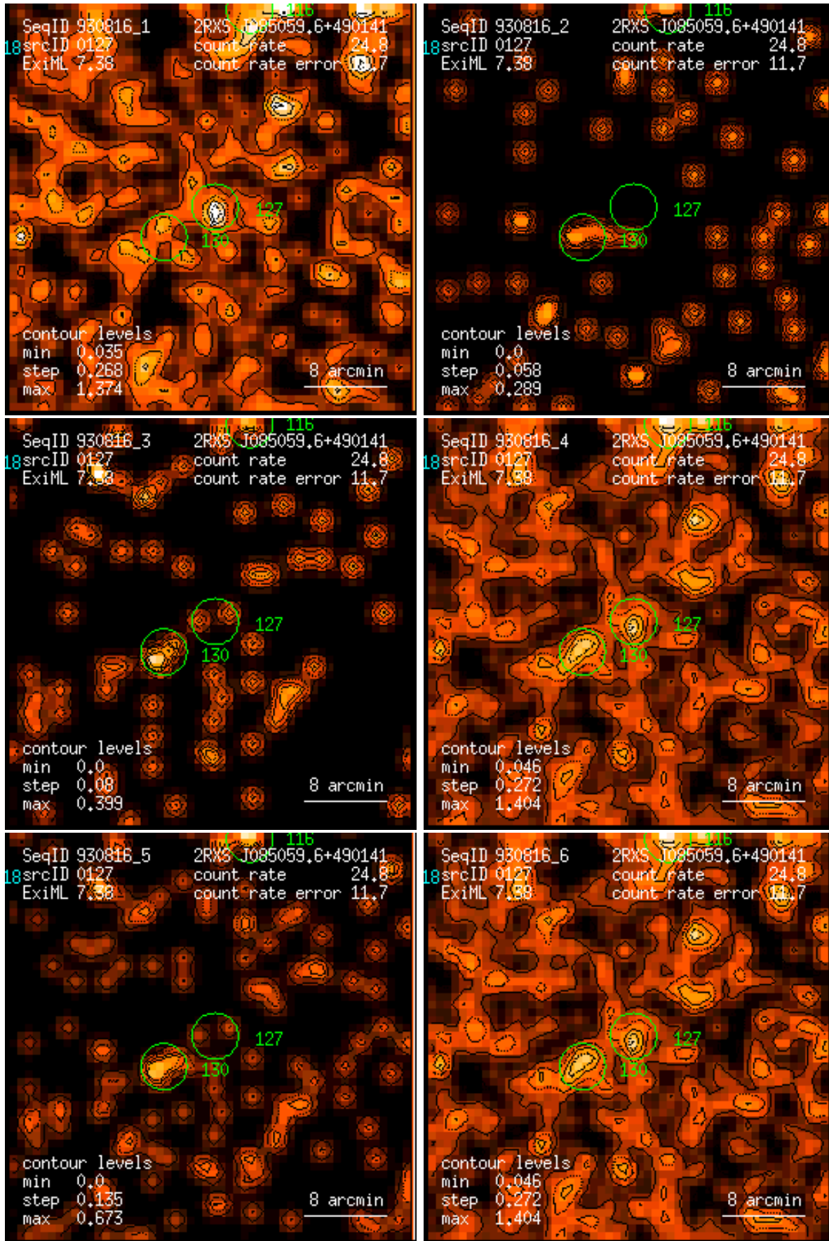
Figure 127: RASS 930816: detection 0127: band rate images, Gaussian filter: (1) PSPC channels 11 – 41, (2) 52 – 90, (3) 91 – 201, (4) 11 – 235, (5) 52 – 201, (6) 11 – 201. Broad band rates in counts/ks. Band rate contour levels in counts/ks/arcmin 2 .
