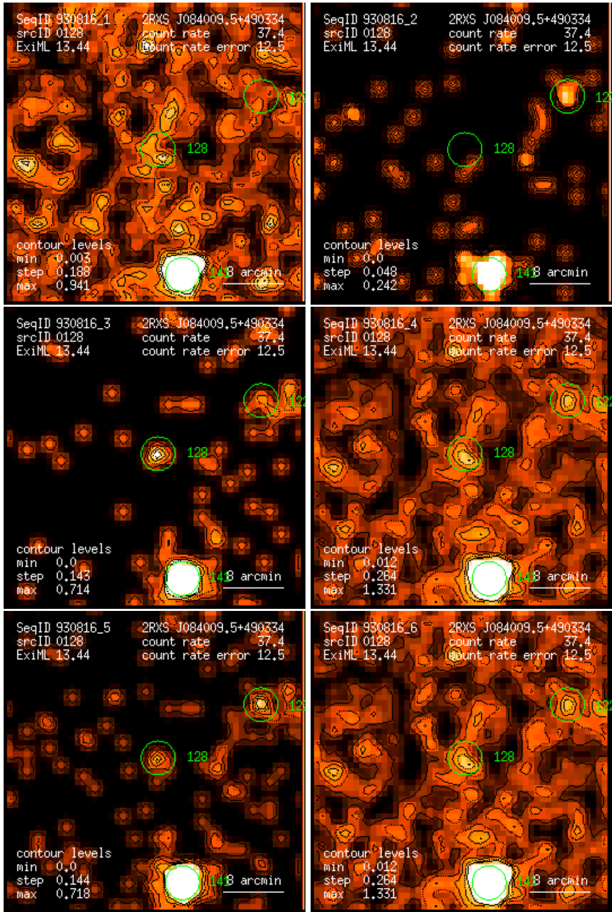
Figure 128: RASS 930816: detection 0128: band rate images, Gaussian filter: (1) PSPC channels 11 – 41, (2) 52 – 90, (3) 91 – 201, (4) 11 – 235, (5) 52 – 201, (6) 11 – 201. Broad band rates in counts/ks. Band rate contour levels in counts/ks/arcmin 2 .
