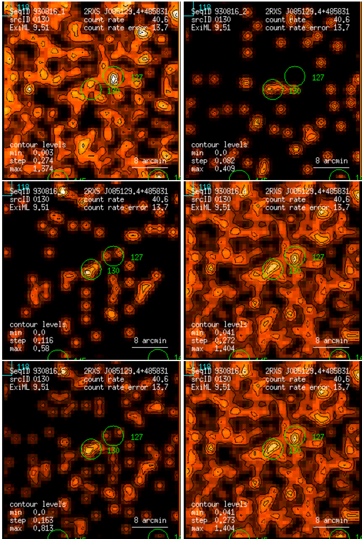
Figure 130: RASS 930816: detection 0130: band rate images, Gaussian filter: (1) PSPC channels 11 – 41, (2) 52 – 90, (3) 91 – 201, (4) 11 – 235, (5) 52 – 201, (6) 11 – 201. Broad band rates in counts/ks. Band rate contour levels in counts/ks/arcmin 2 .
