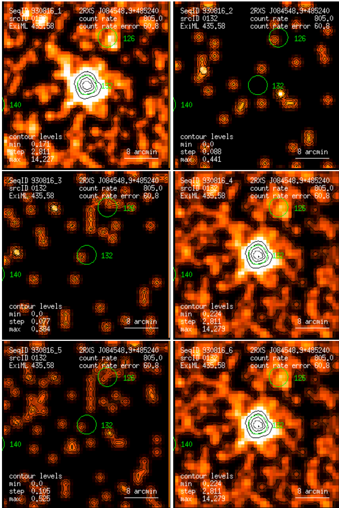
Figure 132: RASS 930816: detection 0132: band rate images, Gaussian filter: (1) PSPC channels 11 – 41, (2) 52 – 90, (3) 91 – 201, (4) 11 – 235, (5) 52 – 201, (6) 11 – 201. Broad band rates in counts/ks. Band rate contour levels in counts/ks/arcmin 2 .
