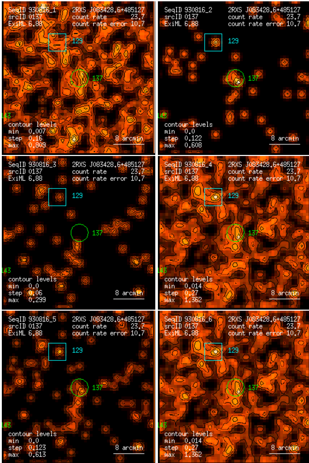
Figure 137: RASS 930816: detection 0137: band rate images, Gaussian filter: (1) PSPC channels 11 – 41, (2) 52 – 90, (3) 91 – 201, (4) 11 – 235, (5) 52 – 201, (6) 11 – 201. Broad band rates in counts/ks. Band rate contour levels in counts/ks/arcmin 2 .
