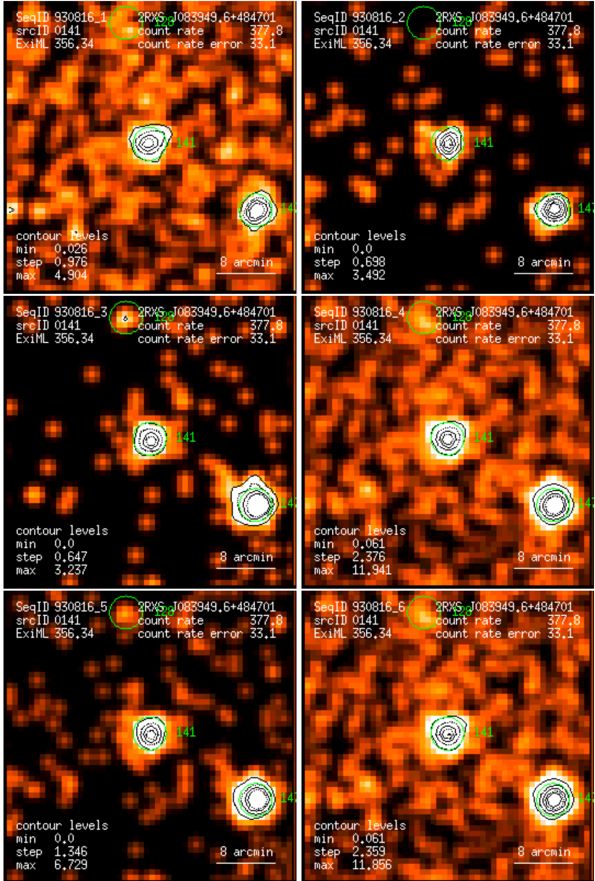
Figure 141: RASS 930816: detection 0141: band rate images, Gaussian filter: (1) PSPC channels 11 – 41, (2) 52 – 90, (3) 91 – 201, (4) 11 – 235, (5) 52 – 201, (6) 11 – 201. Broad band rates in counts/ks. Band rate contour levels in counts/ks/arcmin 2 .
