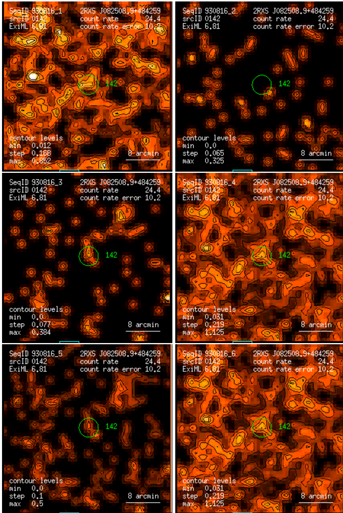
Figure 142: RASS 930816: detection 0142: band rate images, Gaussian filter: (1) PSPC channels 11 – 41, (2) 52 – 90, (3) 91 – 201, (4) 11 – 235, (5) 52 – 201, (6) 11 – 201. Broad band rates in counts/ks. Band rate contour levels in counts/ks/arcmin 2 .
