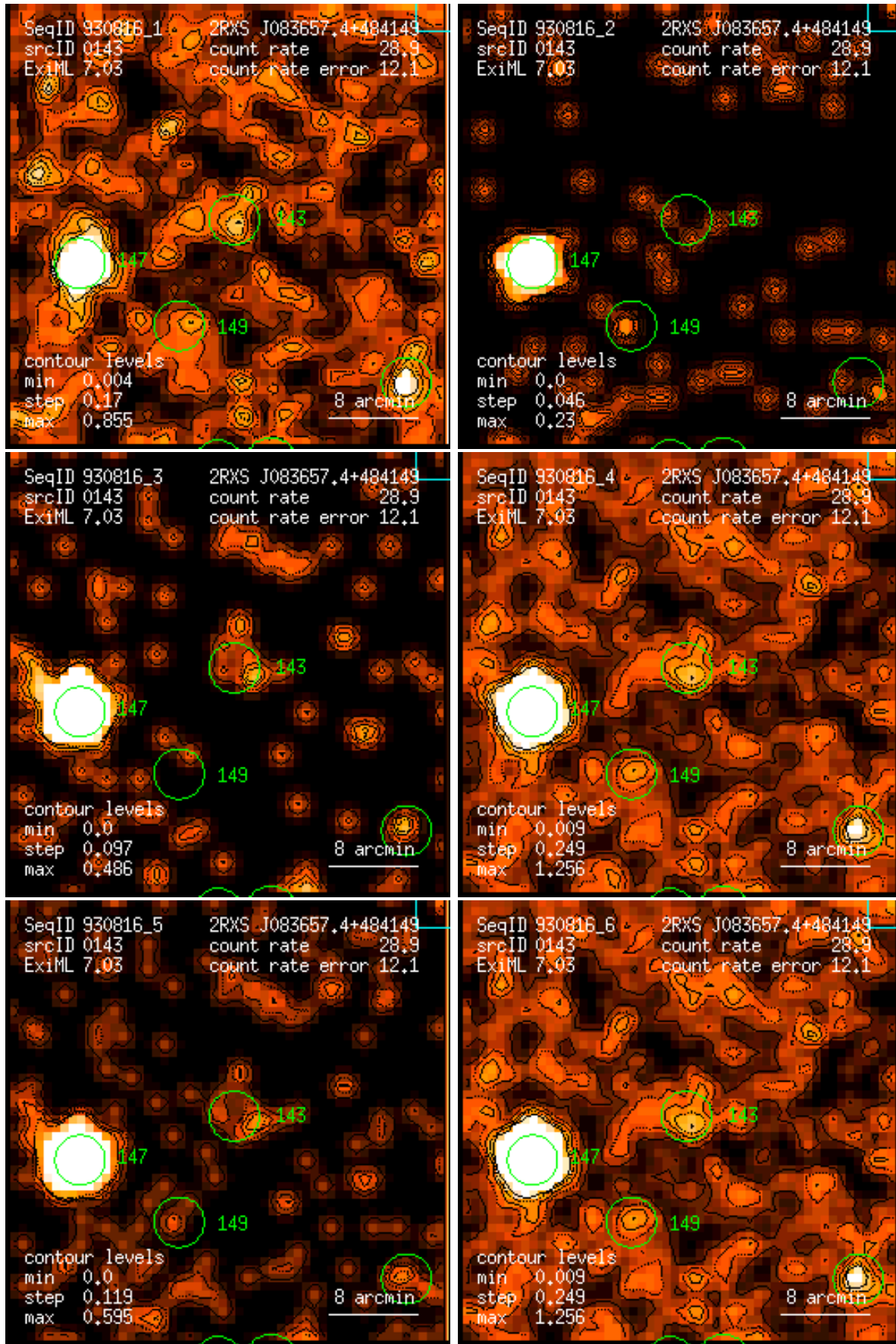
Figure 143: RASS 930816: detection 0143: band rate images, Gaussian filter: (1) PSPC channels 11 – 41, (2) 52 – 90, (3) 91 – 201, (4) 11 – 235, (5) 52 – 201, (6) 11 – 201. Broad band rates in counts/ks. Band rate contour levels in counts/ks/arcmin 2 .
