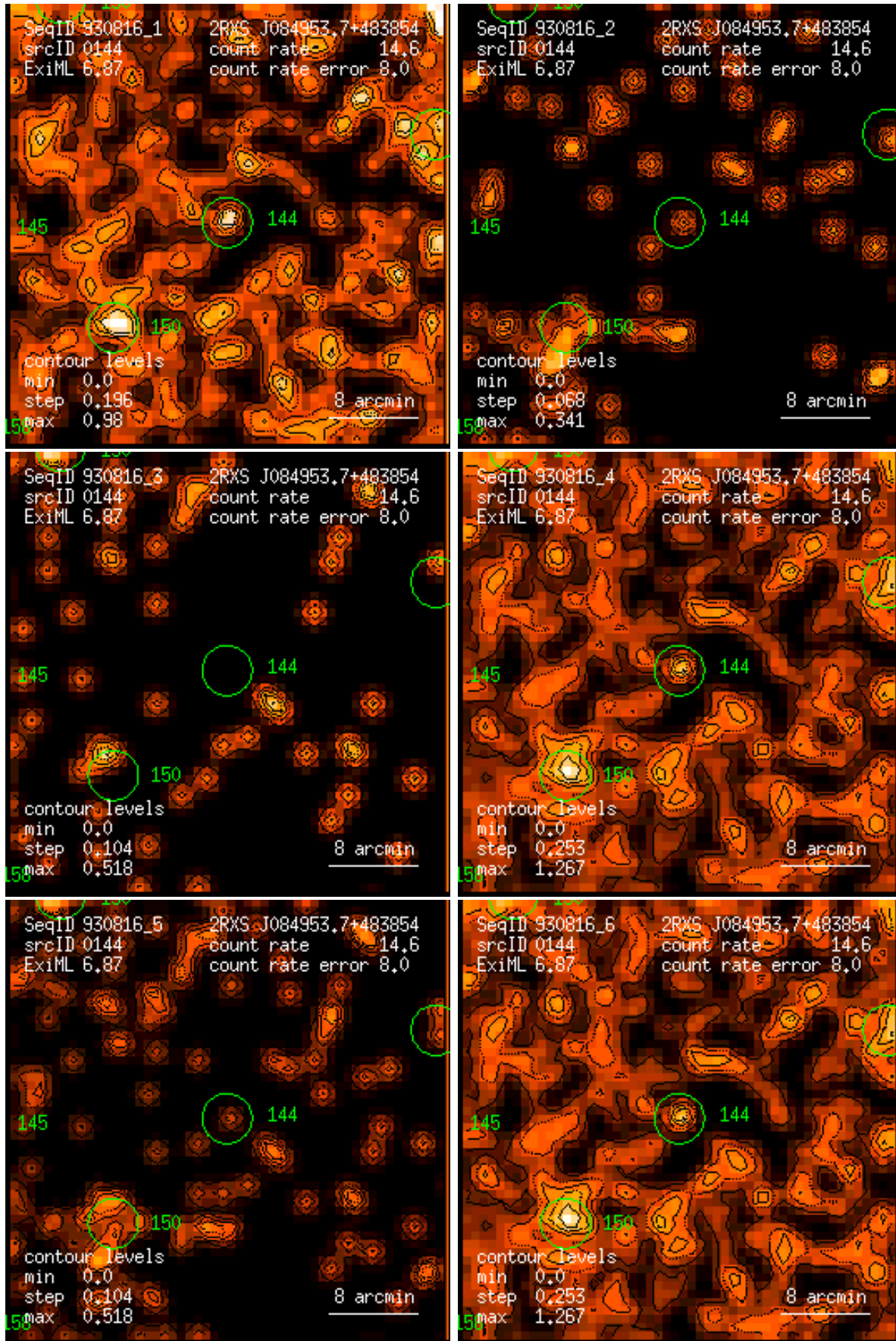
Figure 144: RASS 930816: detection 0144: band rate images, Gaussian filter: (1) PSPC channels 11 – 41, (2) 52 – 90, (3) 91 – 201, (4) 11 – 235, (5) 52 – 201, (6) 11 – 201. Broad band rates in counts/ks. Band rate contour levels in counts/ks/arcmin 2 .
