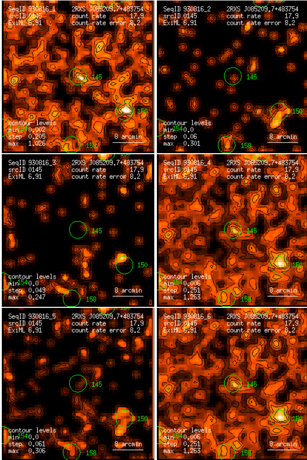
Figure 145: RASS 930816: detection 0145: band rate images, Gaussian filter: (1) PSPC channels 11 – 41, (2) 52 – 90, (3) 91 – 201, (4) 11 – 235, (5) 52 – 201, (6) 11 – 201. Broad band rates in counts/ks. Band rate contour levels in counts/ks/arcmin 2 .
