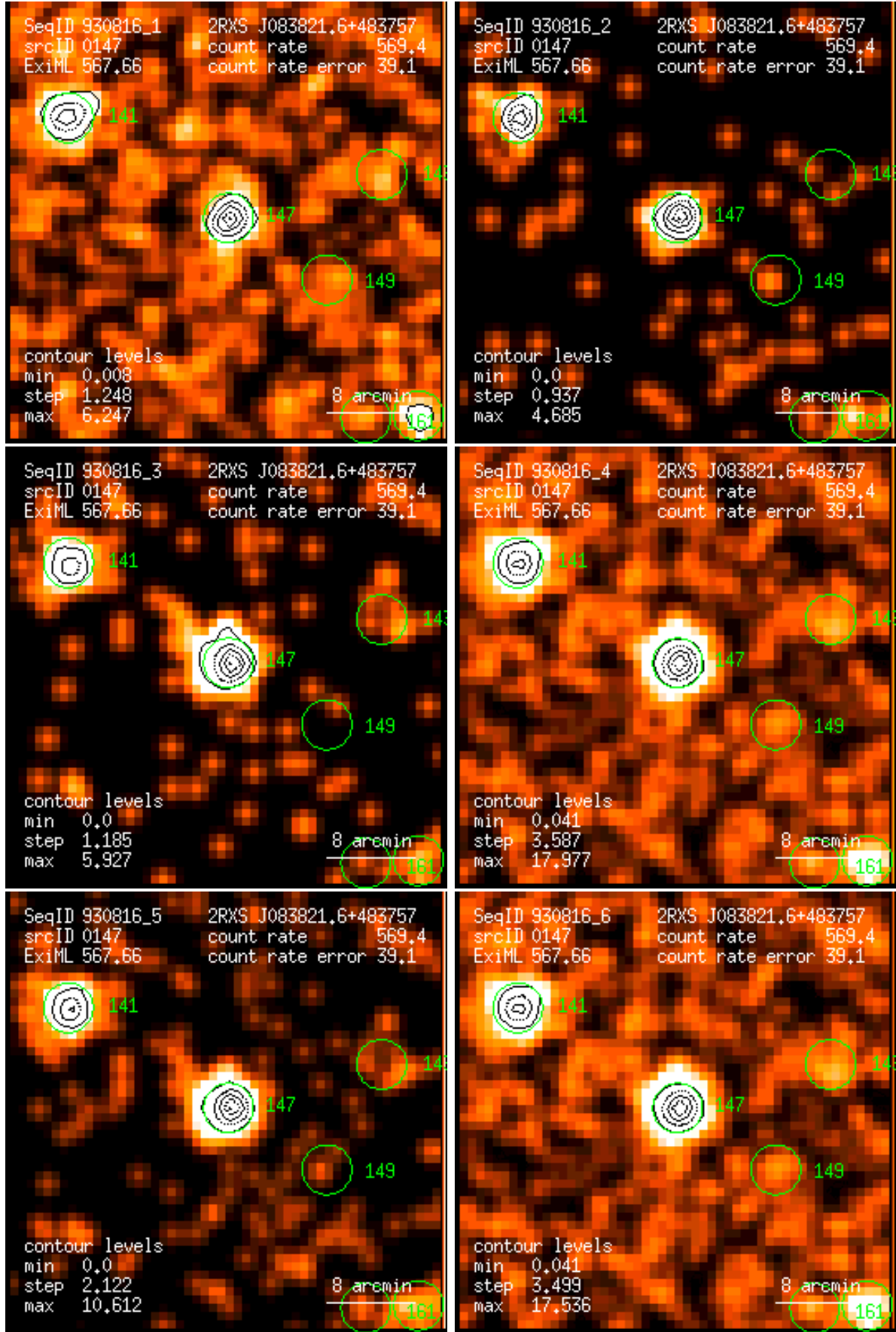
Figure 147: RASS 930816: detection 0147: band rate images, Gaussian filter: (1) PSPC channels 11 – 41, (2) 52 – 90, (3) 91 – 201, (4) 11 – 235, (5) 52 – 201, (6) 11 – 201. Broad band rates in counts/ks. Band rate contour levels in counts/ks/arcmin 2 .
