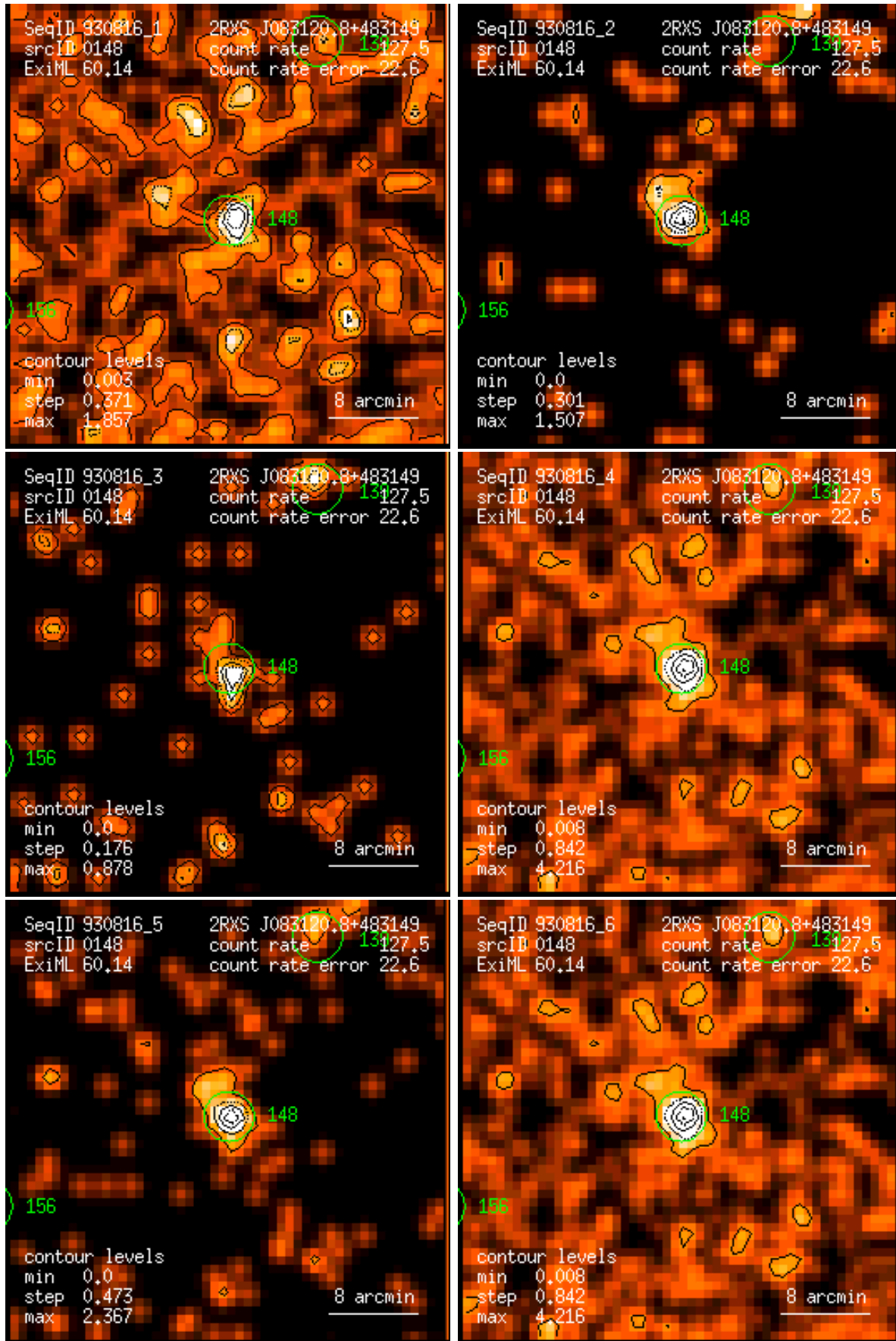
Figure 148: RASS 930816: detection 0148: band rate images, Gaussian filter: (1) PSPC channels 11 – 41, (2) 52 – 90, (3) 91 – 201, (4) 11 – 235, (5) 52 – 201, (6) 11 – 201. Broad band rates in counts/ks. Band rate contour levels in counts/ks/arcmin 2 .
