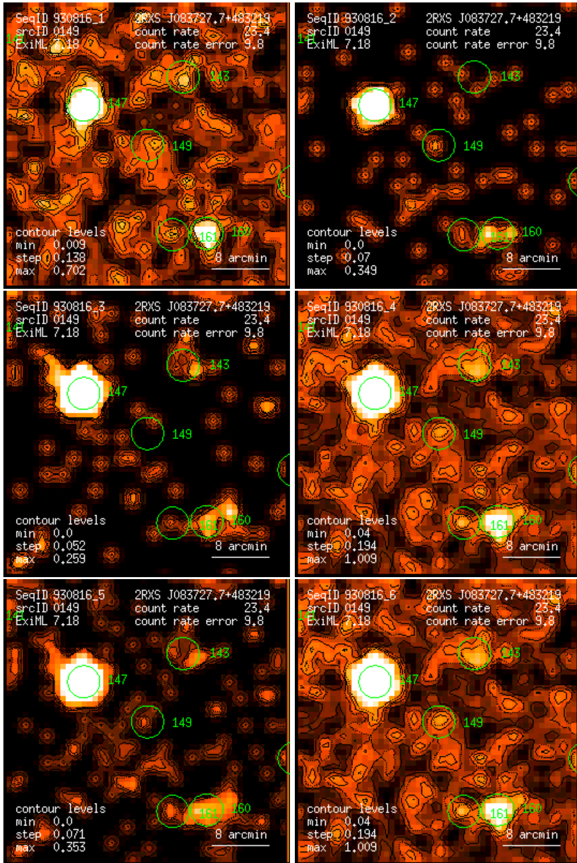
Figure 149: RASS 930816: detection 0149: band rate images, Gaussian filter: (1) PSPC channels 11 – 41, (2) 52 – 90, (3) 91 – 201, (4) 11 – 235, (5) 52 – 201, (6) 11 – 201. Broad band rates in counts/ks. Band rate contour levels in counts/ks/arcmin 2 .
