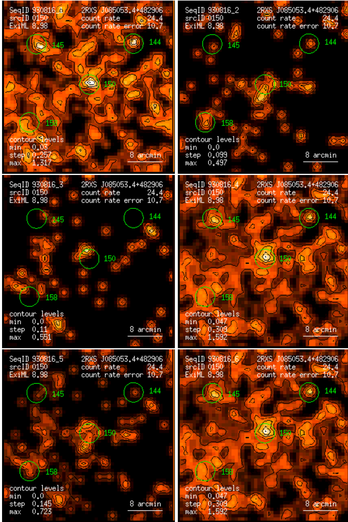
Figure 150: RASS 930816: detection 0150: band rate images, Gaussian filter: (1) PSPC channels 11 – 41, (2) 52 – 90, (3) 91 – 201, (4) 11 – 235, (5) 52 – 201, (6) 11 – 201. Broad band rates in counts/ks. Band rate contour levels in counts/ks/arcmin 2 .
