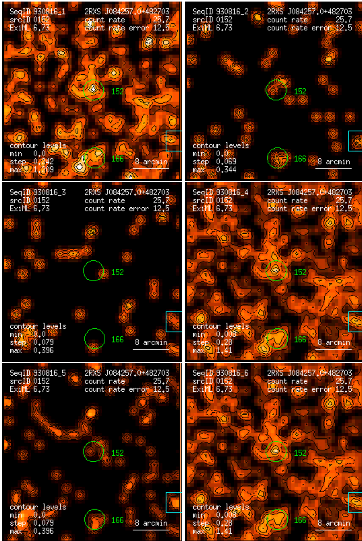
Figure 152: RASS 930816: detection 0152: band rate images, Gaussian filter: (1) PSPC channels 11 – 41, (2) 52 – 90, (3) 91 – 201, (4) 11 – 235, (5) 52 – 201, (6) 11 – 201. Broad band rates in counts/ks. Band rate contour levels in counts/ks/arcmin 2 .
