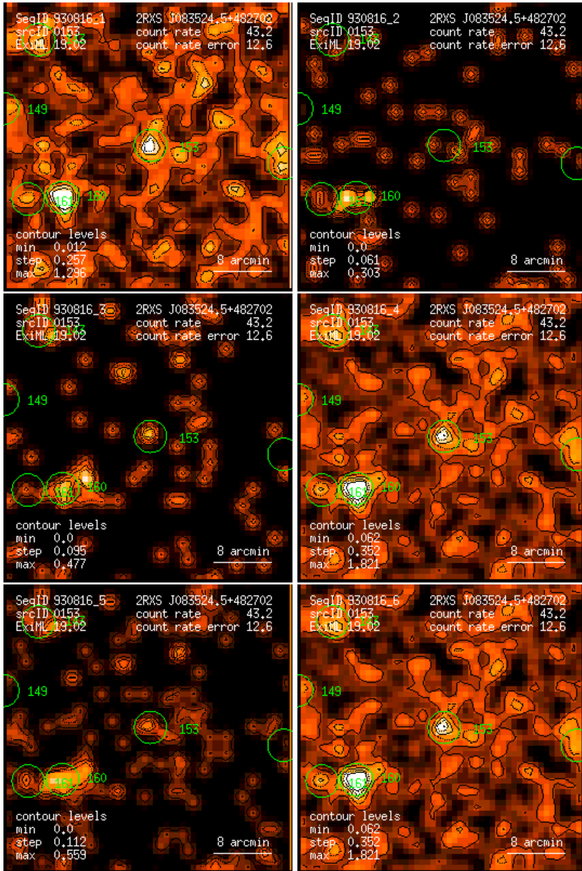
Figure 153: RASS 930816: detection 0153: band rate images, Gaussian filter: (1) PSPC channels 11 – 41, (2) 52 – 90, (3) 91 – 201, (4) 11 – 235, (5) 52 – 201, (6) 11 – 201. Broad band rates in counts/ks. Band rate contour levels in counts/ks/arcmin 2 .
