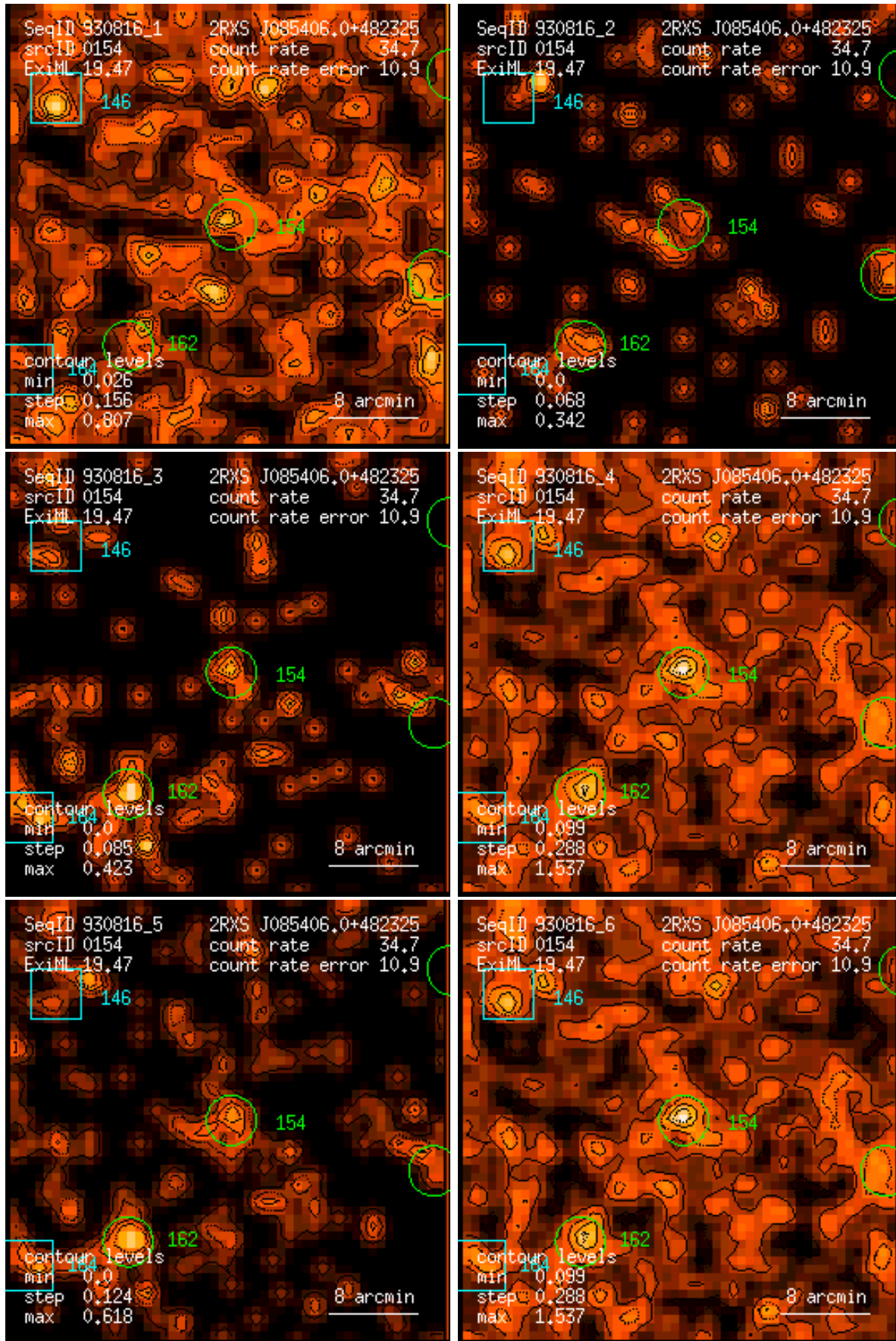
Figure 154: RASS 930816: detection 0154: band rate images, Gaussian filter: (1) PSPC channels 11 – 41, (2) 52 – 90, (3) 91 – 201, (4) 11 – 235, (5) 52 – 201, (6) 11 – 201. Broad band rates in counts/ks. Band rate contour levels in counts/ks/arcmin 2 .
