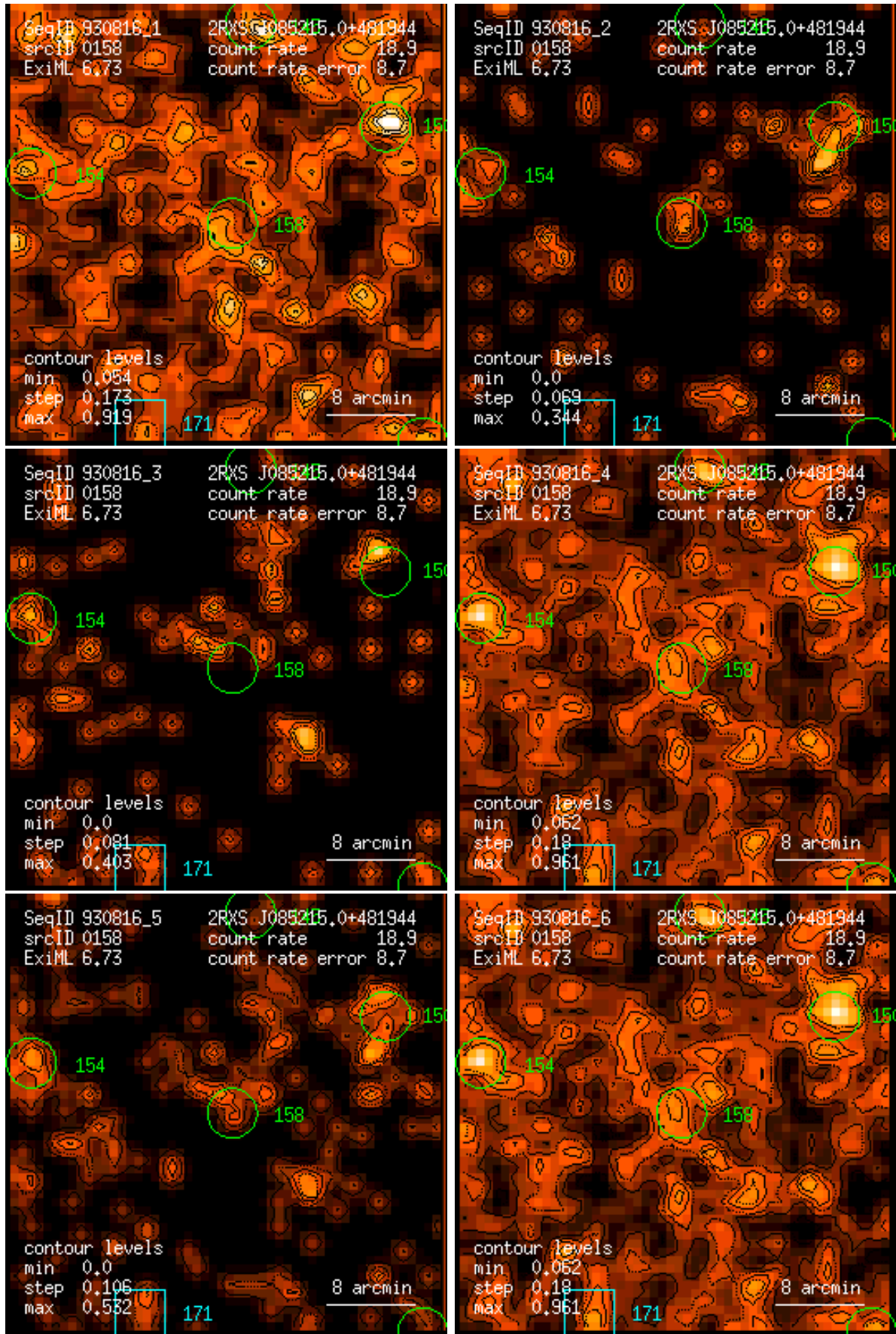
Figure 158: RASS 930816: detection 0158: band rate images, Gaussian filter: (1) PSPC channels 11 – 41, (2) 52 – 90, (3) 91 – 201, (4) 11 – 235, (5) 52 – 201, (6) 11 – 201. Broad band rates in counts/ks. Band rate contour levels in counts/ks/arcmin 2 .
