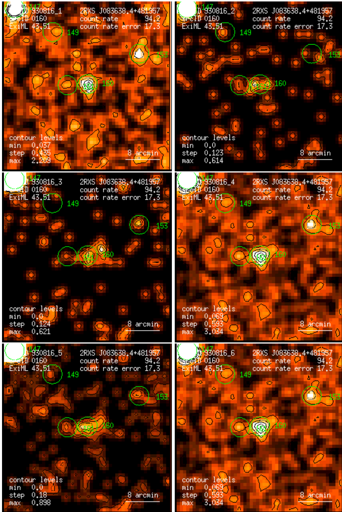
Figure 160: RASS 930816: detection 0160: band rate images, Gaussian filter: (1) PSPC channels 11 – 41, (2) 52 – 90, (3) 91 – 201, (4) 11 – 235, (5) 52 – 201, (6) 11 – 201. Broad band rates in counts/ks. Band rate contour levels in counts/ks/arcmin 2 .
