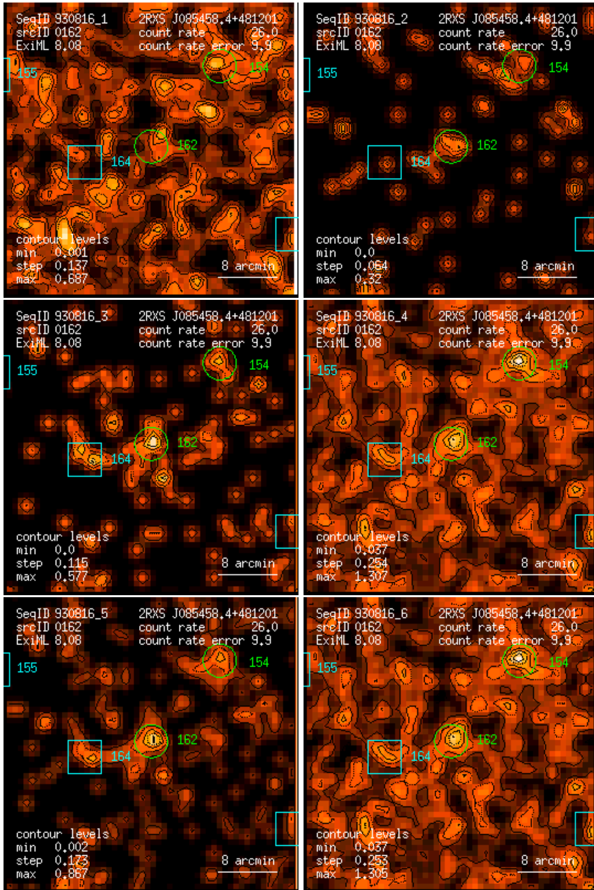
Figure 162: RASS 930816: detection 0162: band rate images, Gaussian filter: (1) PSPC channels 11 – 41, (2) 52 – 90, (3) 91 – 201, (4) 11 – 235, (5) 52 – 201, (6) 11 – 201. Broad band rates in counts/ks. Band rate contour levels in counts/ks/arcmin 2 .
