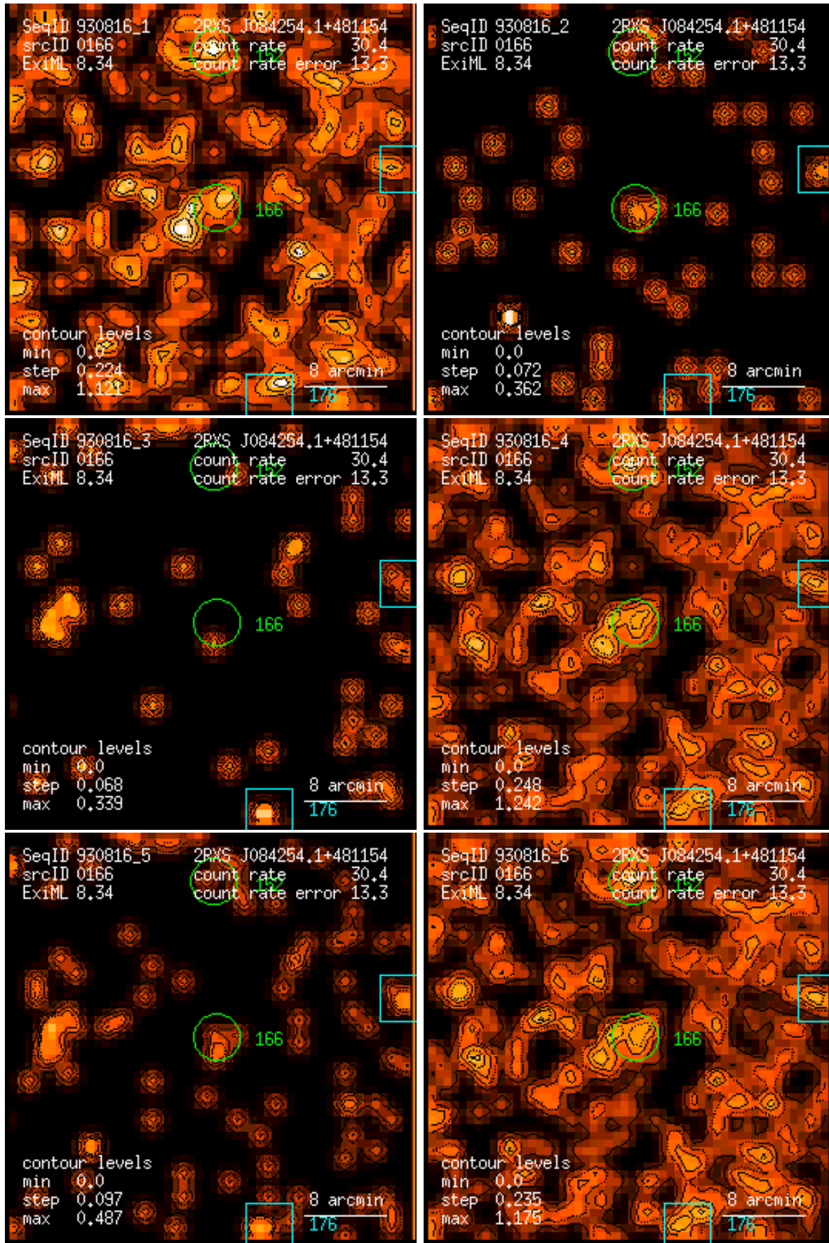
Figure 166: RASS 930816: detection 0166: band rate images, Gaussian filter: (1) PSPC channels 11 – 41, (2) 52 – 90, (3) 91 – 201, (4) 11 – 235, (5) 52 – 201, (6) 11 – 201. Broad band rates in counts/ks. Band rate contour levels in counts/ks/arcmin 2 .
