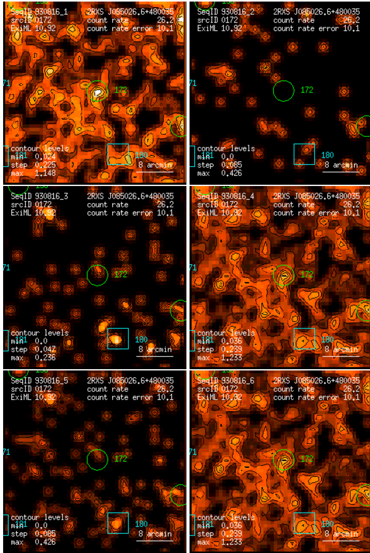
Figure 172: RASS 930816: detection 0172: band rate images, Gaussian filter: (1) PSPC channels 11 – 41, (2) 52 – 90, (3) 91 – 201, (4) 11 – 235, (5) 52 – 201, (6) 11 – 201. Broad band rates in counts/ks. Band rate contour levels in counts/ks/arcmin 2 .
