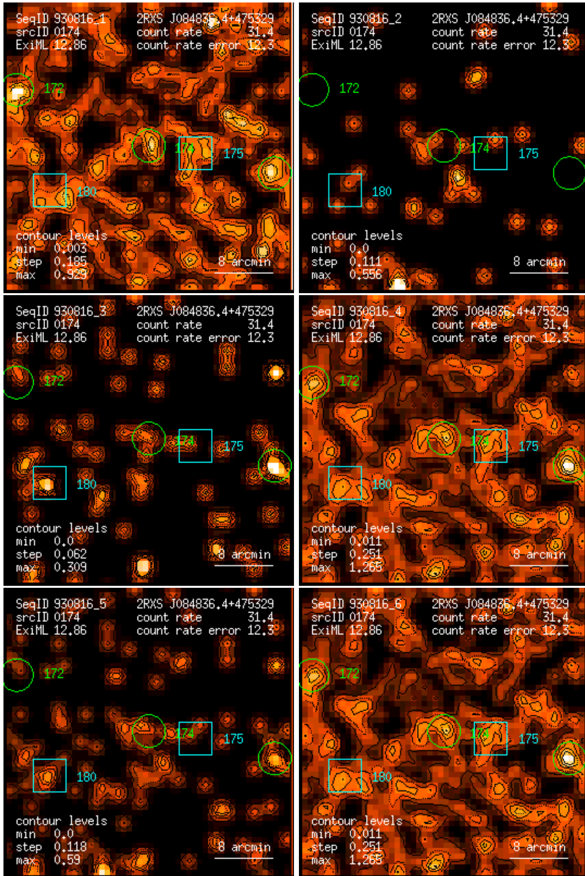
Figure 174: RASS 930816: detection 0174: band rate images, Gaussian filter: (1) PSPC channels 11 – 41, (2) 52 – 90, (3) 91 – 201, (4) 11 – 235, (5) 52 – 201, (6) 11 – 201. Broad band rates in counts/ks. Band rate contour levels in counts/ks/arcmin 2 .
