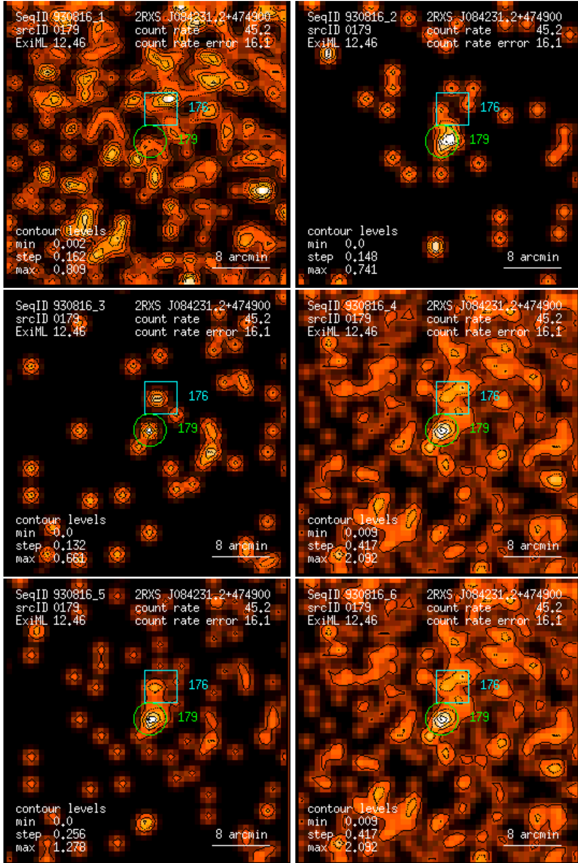
Figure 179: RASS 930816: detection 0179: band rate images, Gaussian filter: (1) PSPC channels 11 – 41, (2) 52 – 90, (3) 91 – 201, (4) 11 – 235, (5) 52 – 201, (6) 11 – 201. Broad band rates in counts/ks. Band rate contour levels in counts/ks/arcmin 2 .
